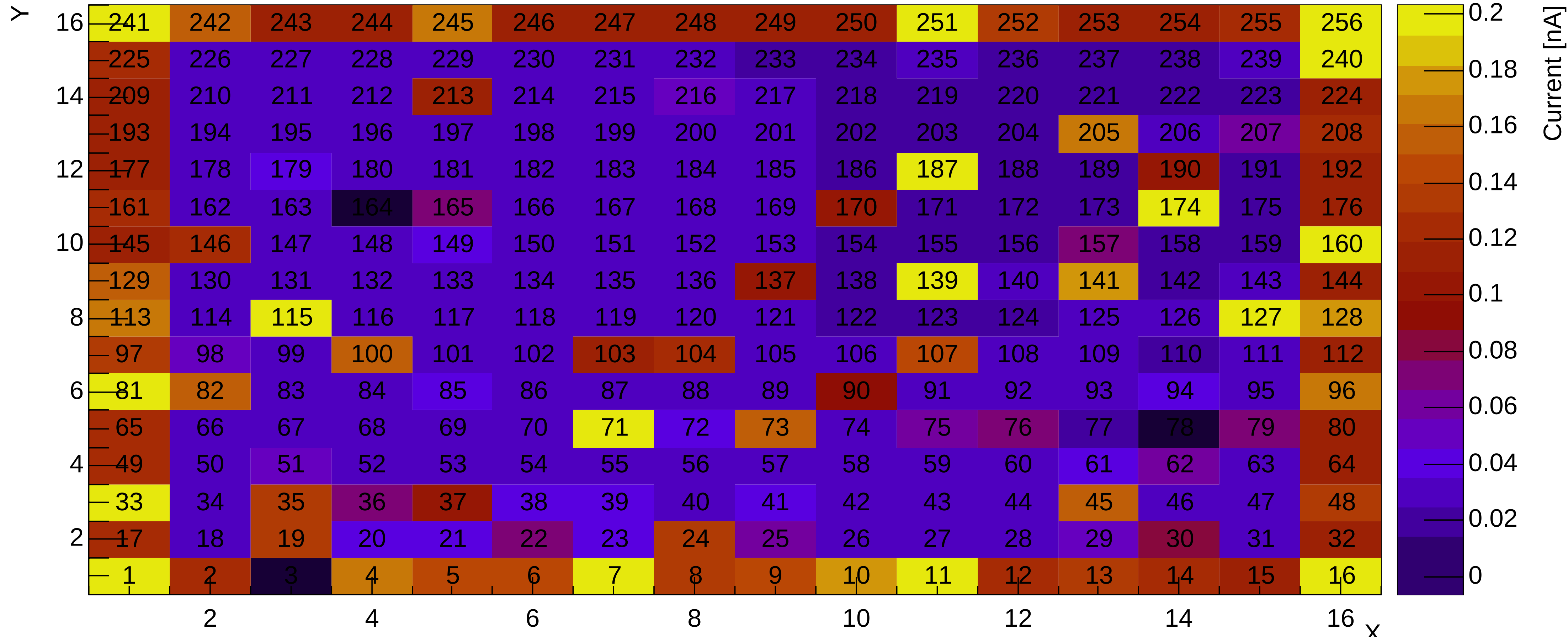
Current at 120 V for sensor 16
