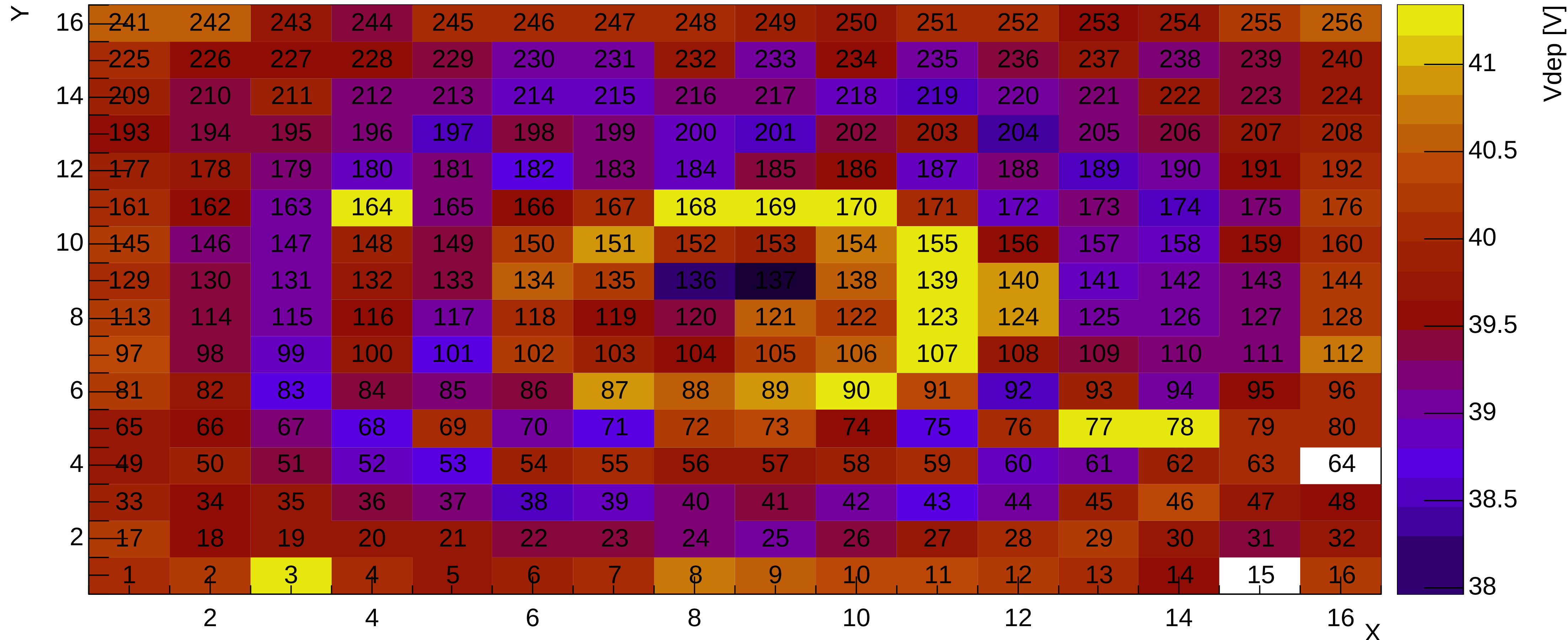
Depletion Voltage for sensor 16
