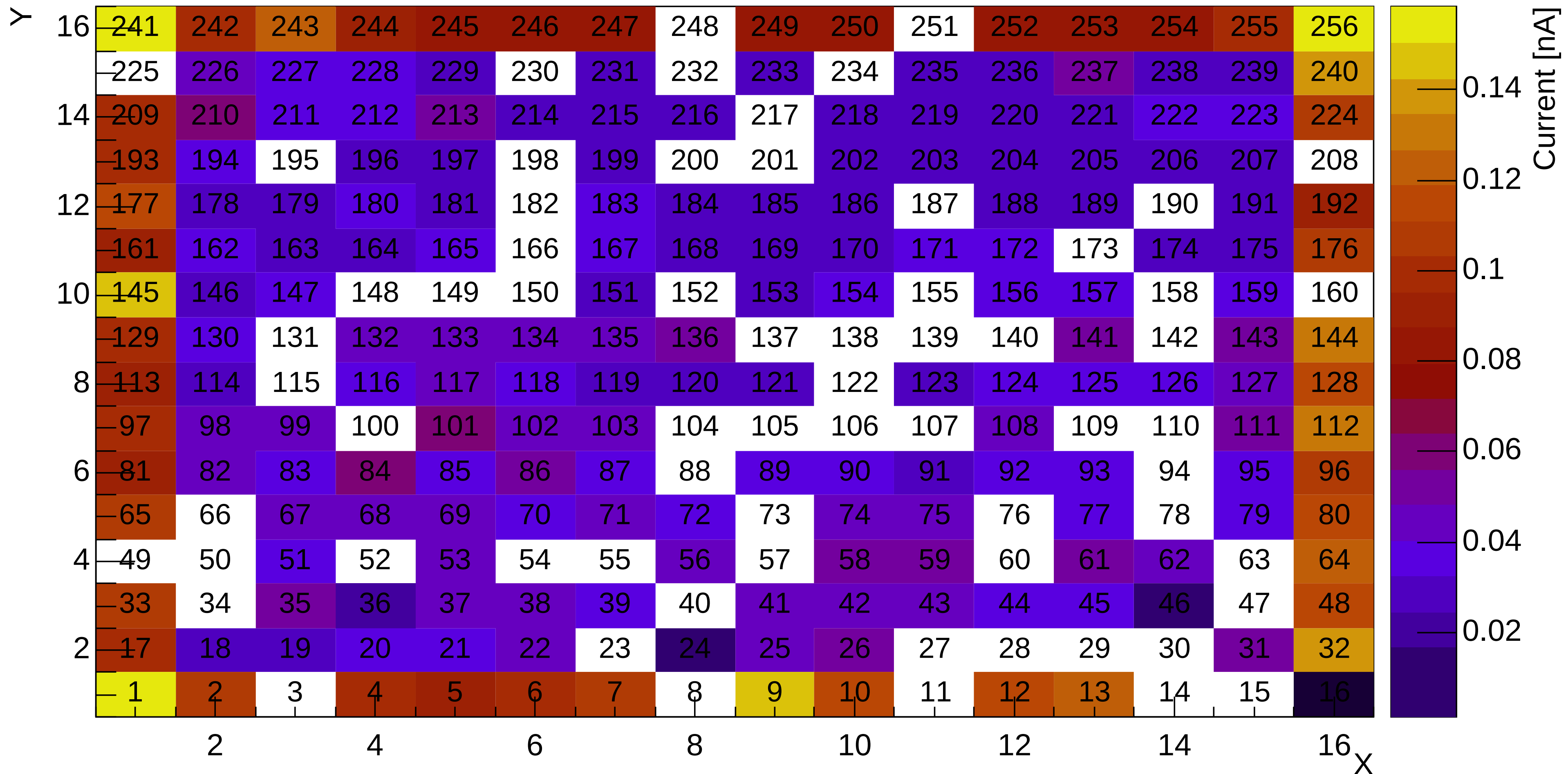
Current at 120 V for sensor CSIS_001
