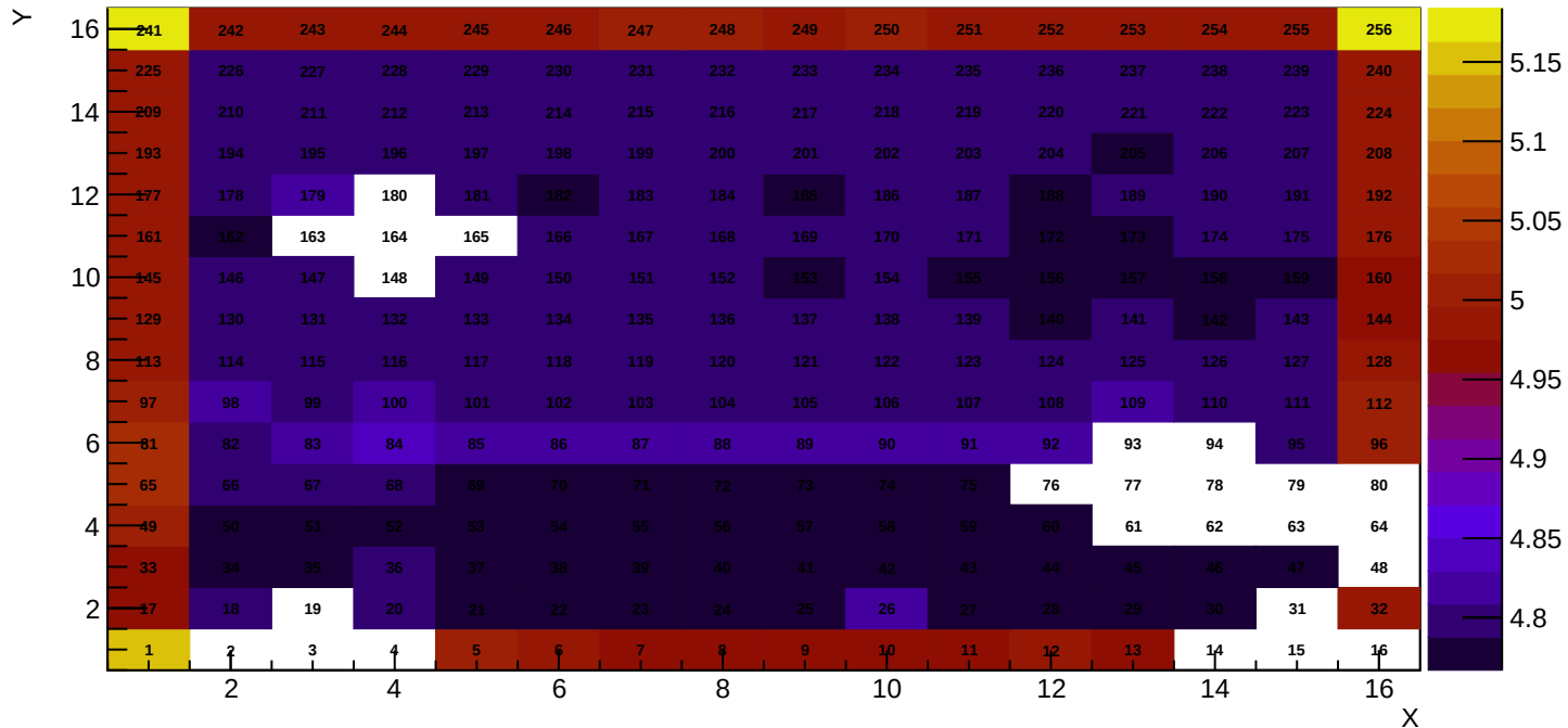
Full depletion capacitance for sensor 16
