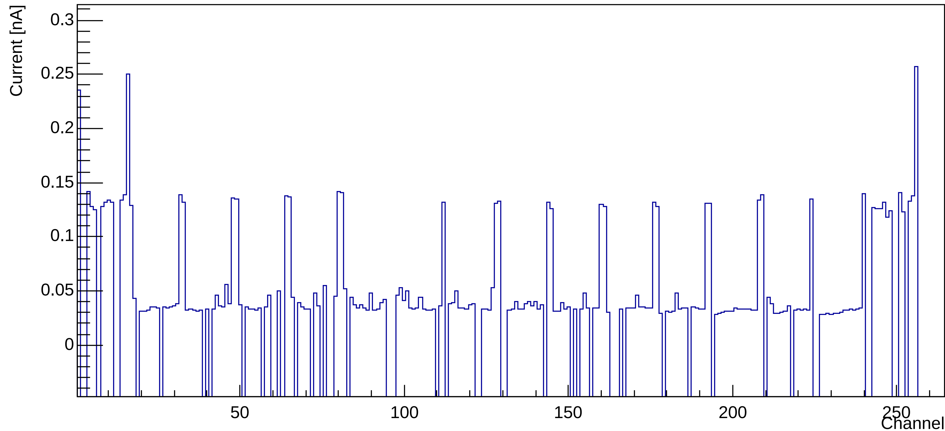
Current per Channel at 120 V
