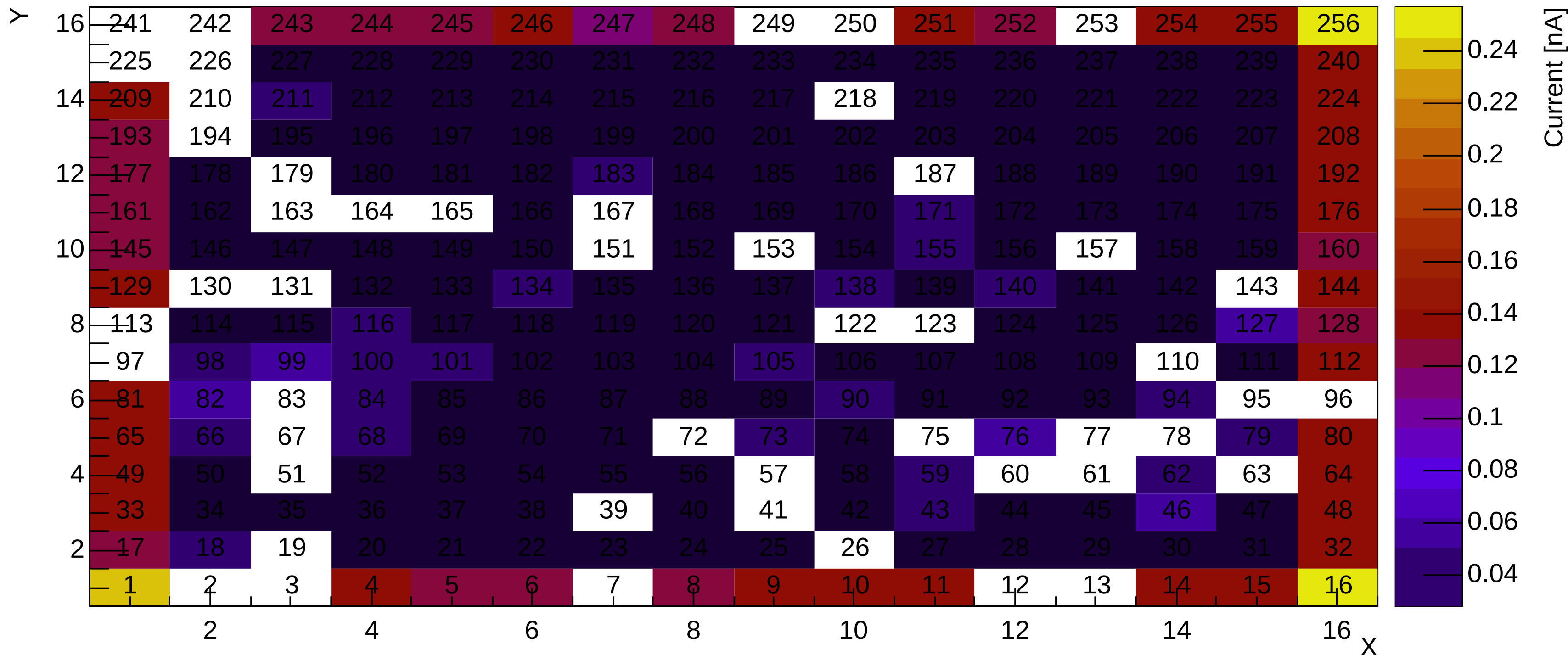
Current at 120 V for sensor 17
