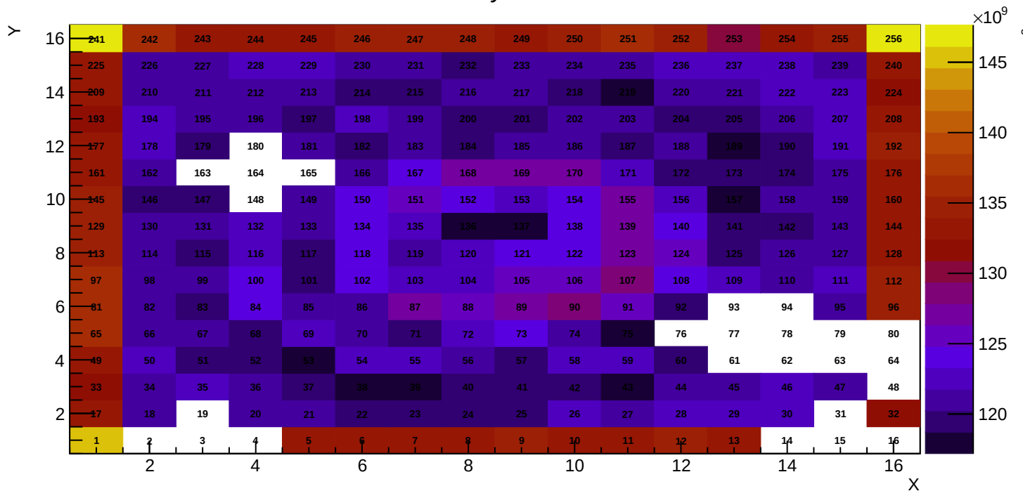
Donnor density for sensor 16
