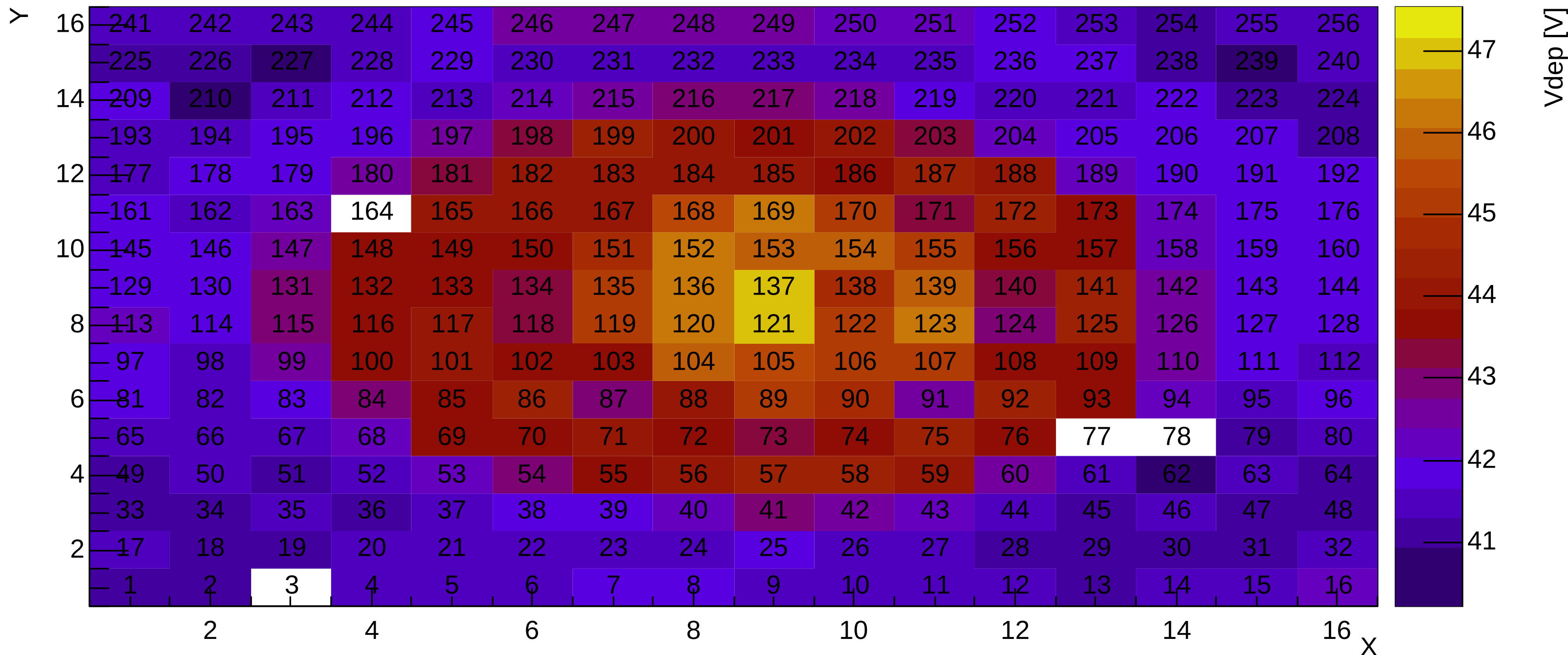
Depletion Voltage for sensor 13
