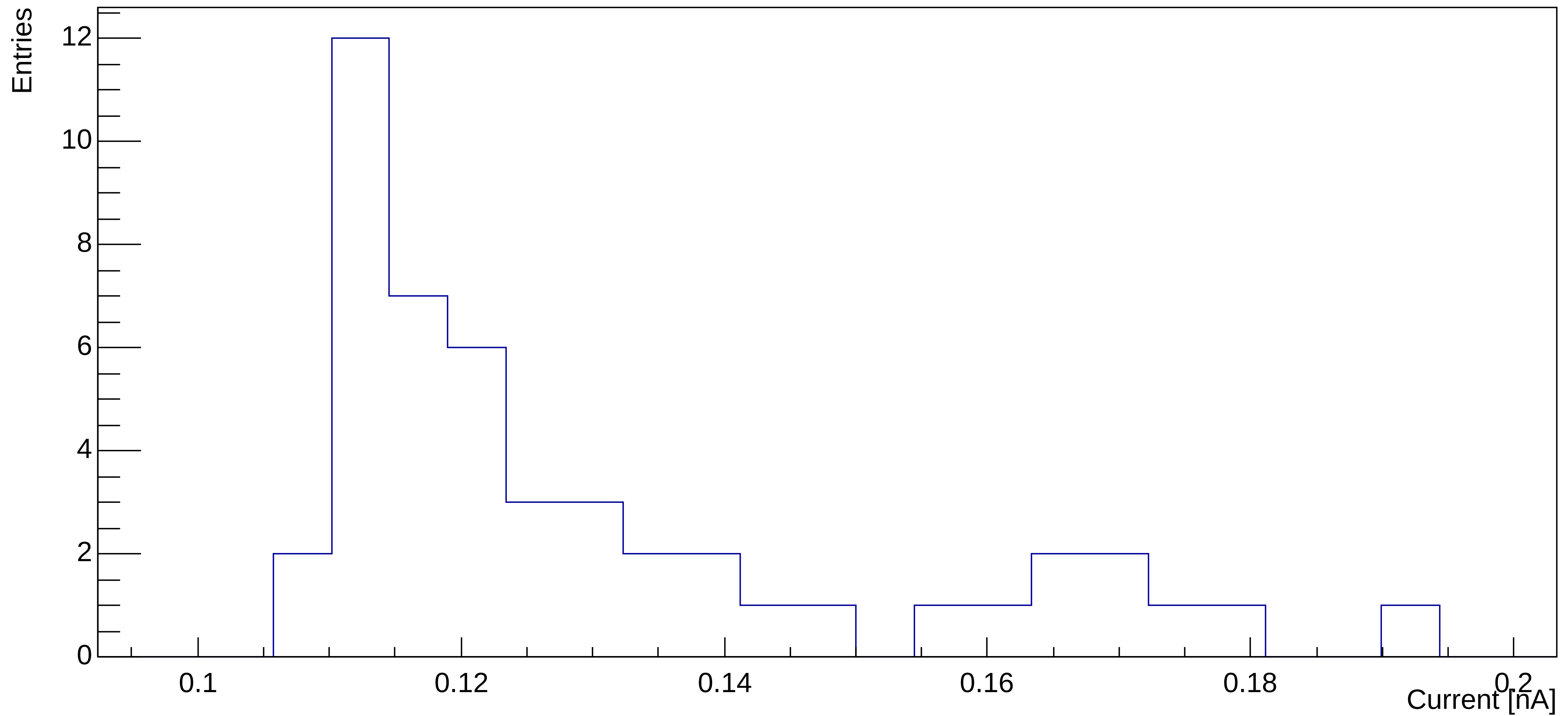
Current distribution at borders zoomed
