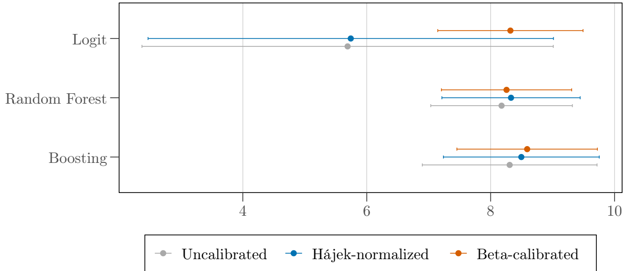
Estimated ATE (AIPW)
