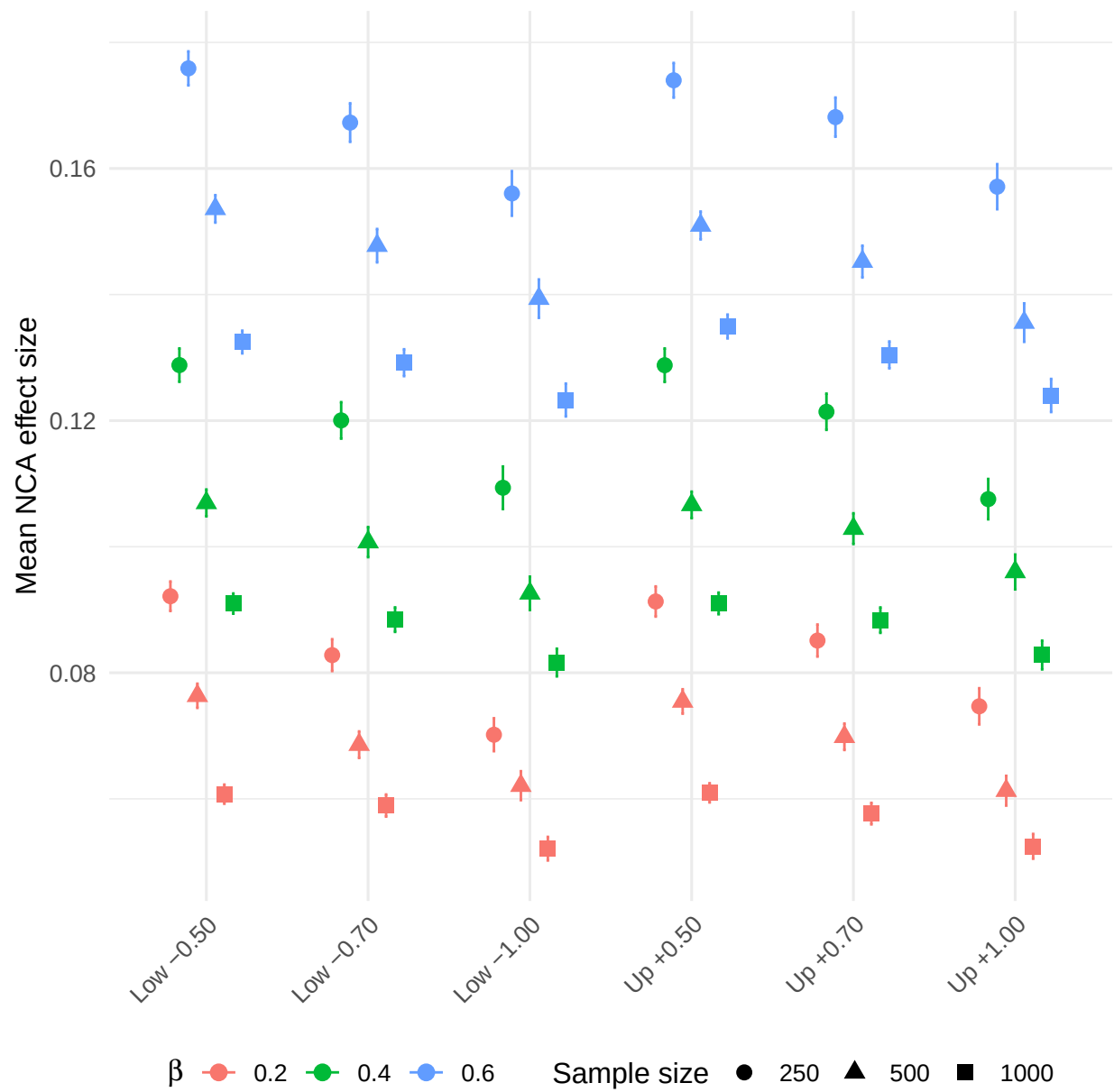
Figure 8 Effects of threshold shifts on observed NCA estimates
