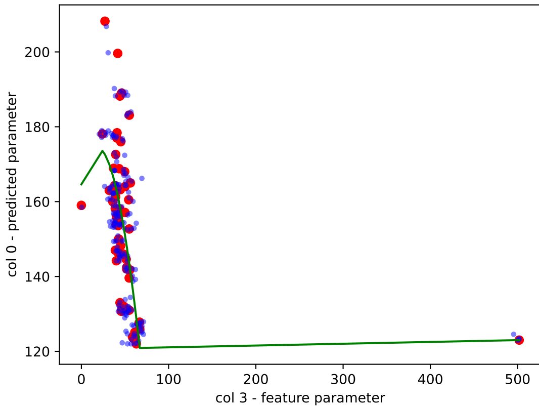
KDE Augmented Data - R^2 = 0.442
