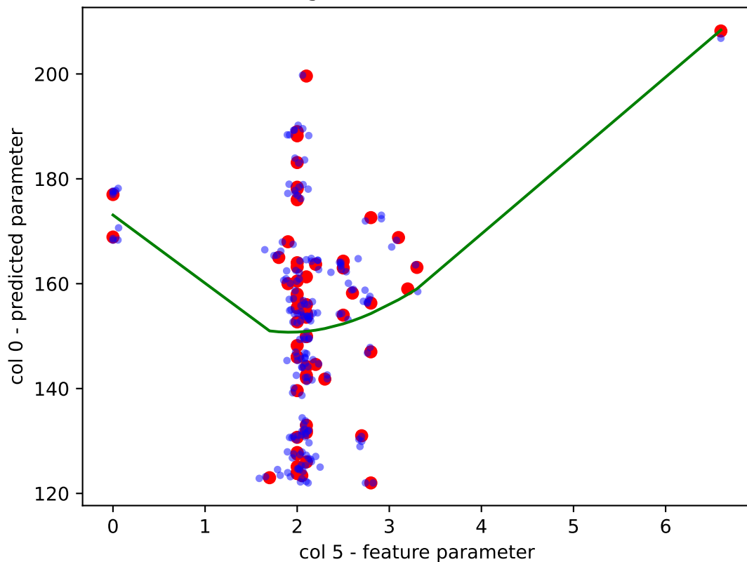
KDE Augmented Data - R^2 = 0.170
