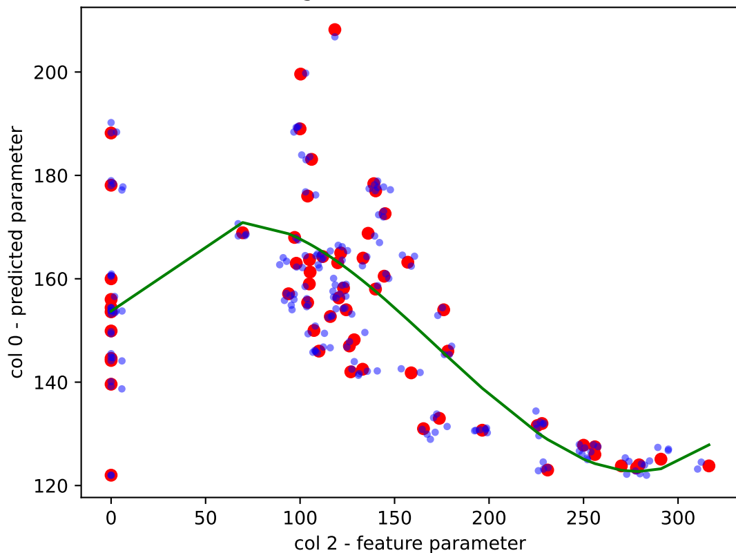
KDE Augmented Data - R^2 = 0.527
