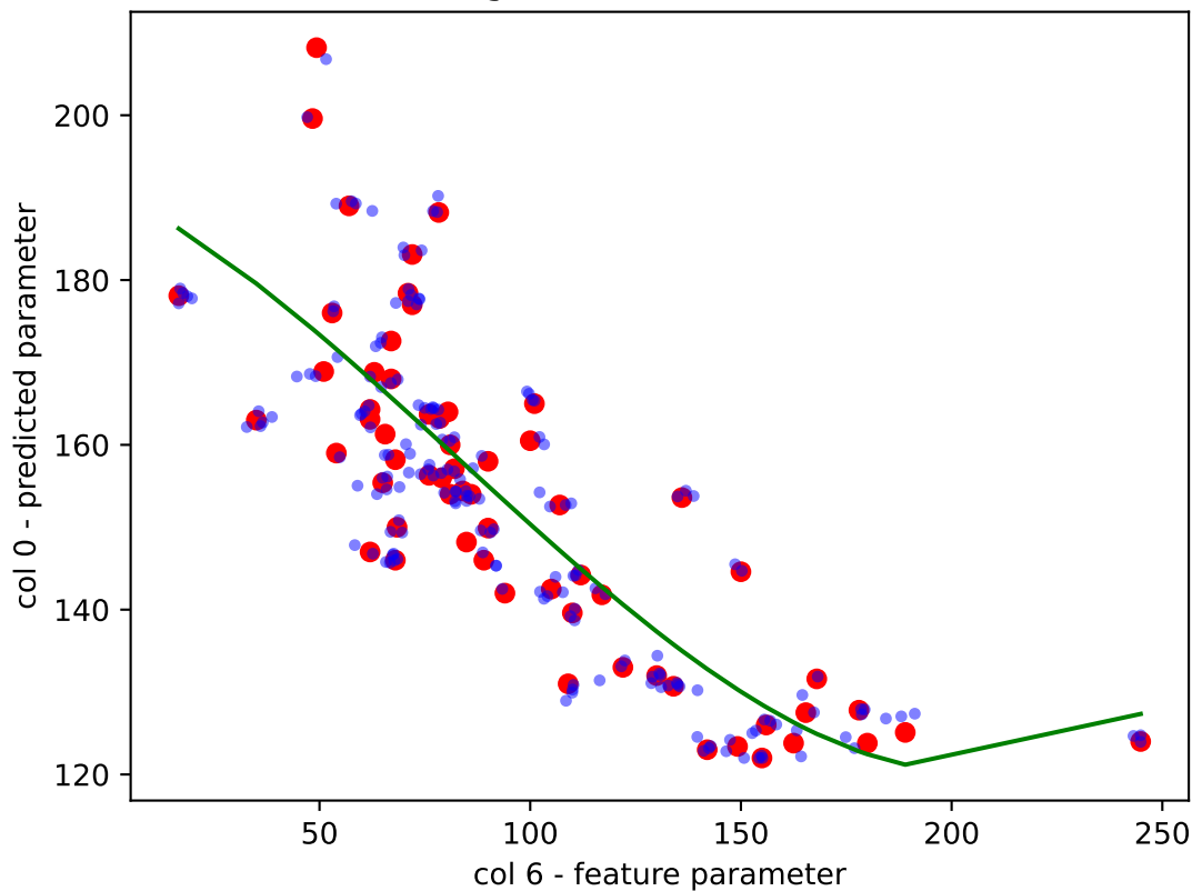
KDE Augmented Data - R^2 = 0.685
