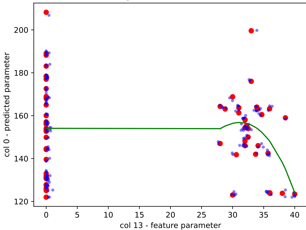
KDE Augmented Data - R^2 = 0.069
