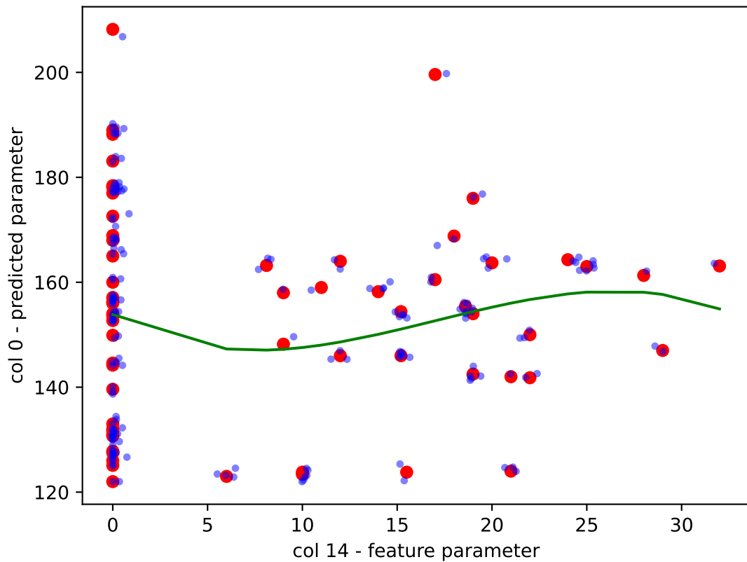
KDE Augmented Data - R^2 = 0.019
