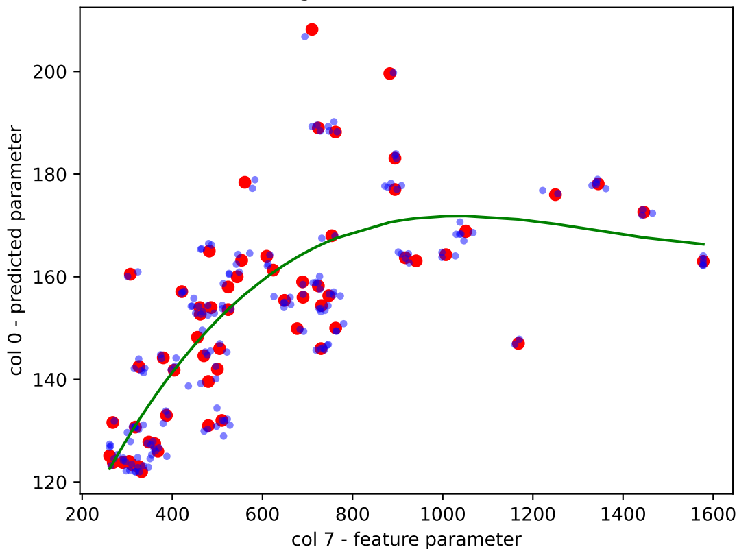
KDE Augmented Data - R^2 = 0.593
