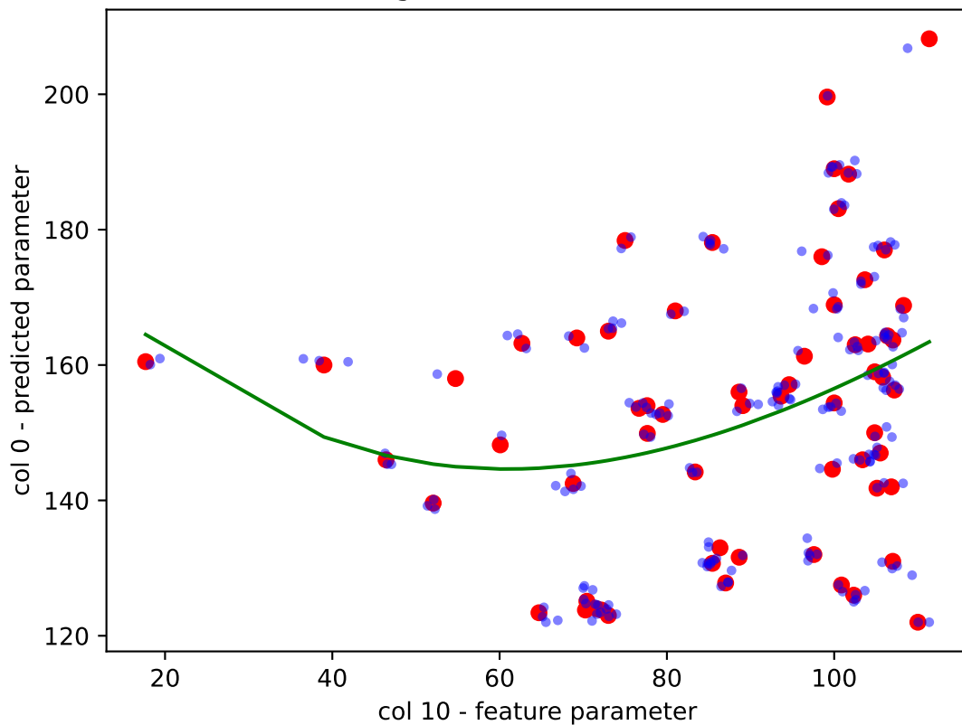
KDE Augmented Data - R^2 = 0.095
