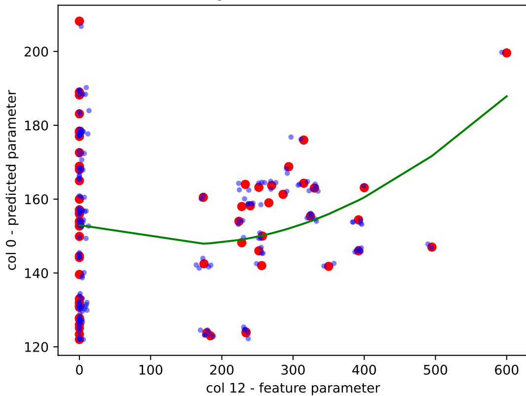
KDE Augmented Data - R^2 = 0.080
