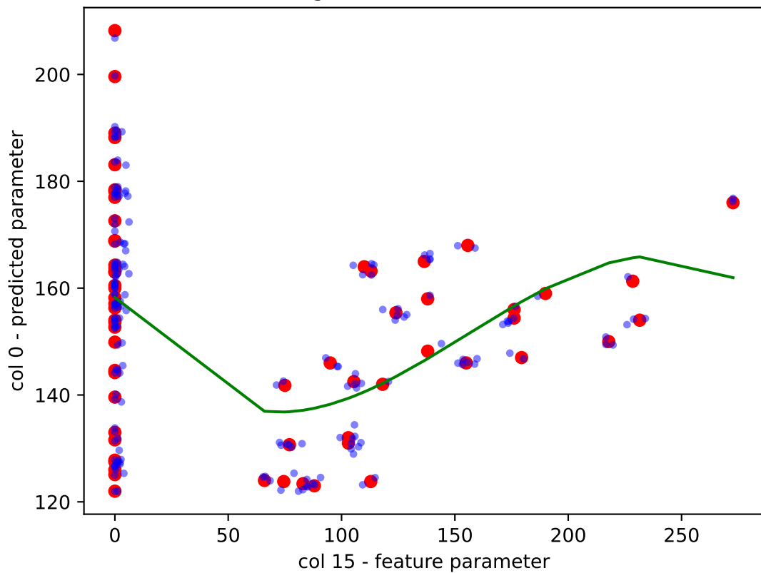
KDE Augmented Data - R^2 = 0.189
