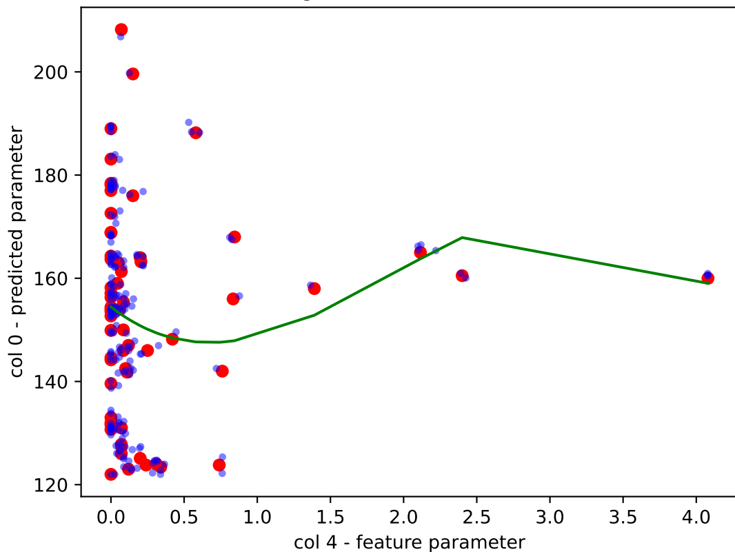
KDE Augmented Data - R^2 = 0.027
