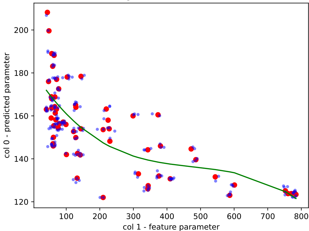
KDE Augmented Data - R^2 = 0.565
