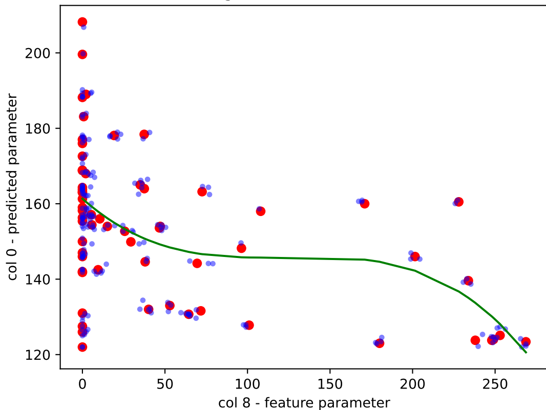
KDE Augmented Data - R^2 = 0.263
