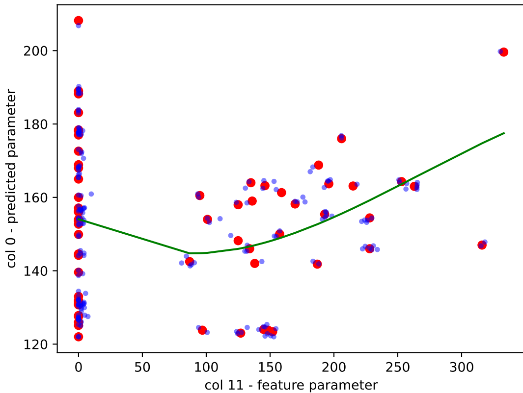
KDE Augmented Data - R^2 = 0.089
