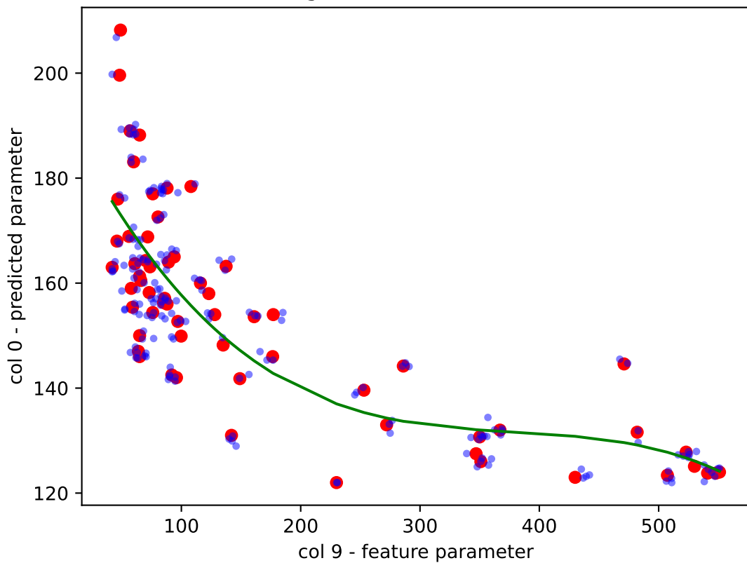
KDE Augmented Data - R^2 = 0.660
