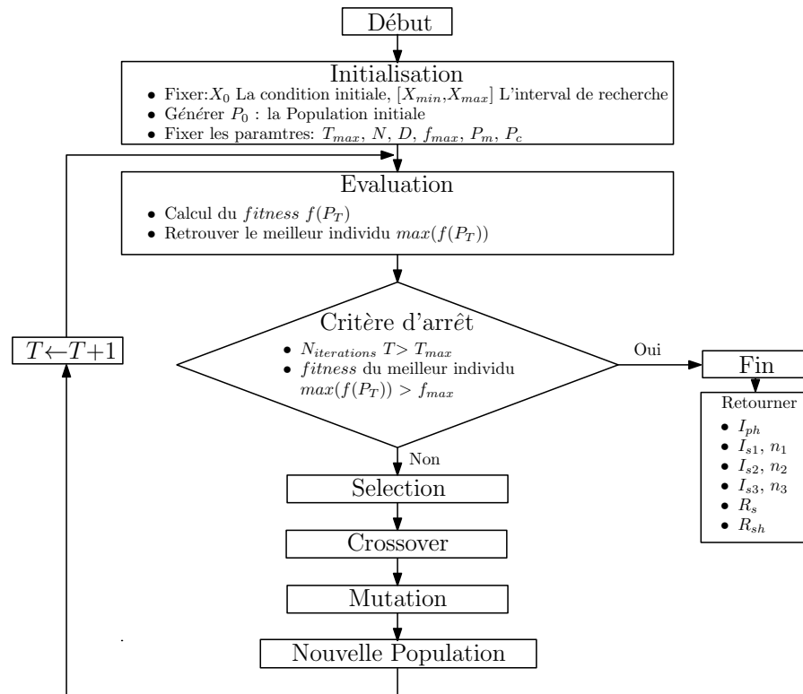
Figure II.16: Algorithme génétique
