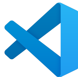
FIGURE 3.2 – logo VsCode
