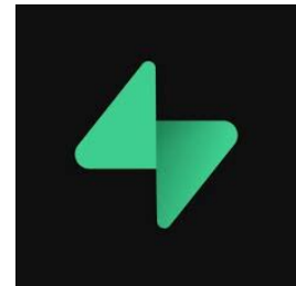
FIGURE 3.6 – Logo Supabase
