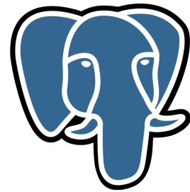
FIGURE 3.14 – Logo PostgreSQL
