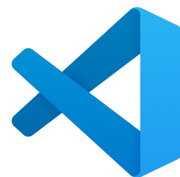
FIGURE 3.2 – logo VsCode
