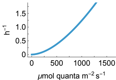
ROS damage rate
