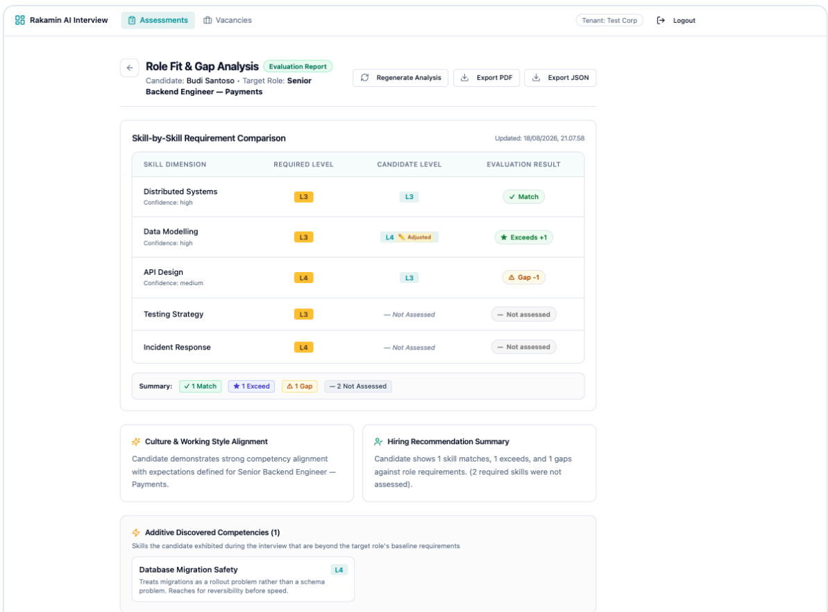
Figure 5.2 — Role Fit & Gap Analysis: Automated delta calculation matrix (Match / Exceeds +1 / Gap -1 / Not Assessed), summary counters, executive culture alignment narrative, and additive discovered competencies.
