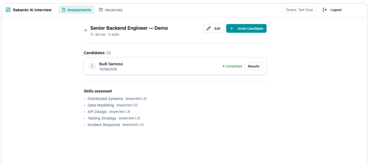
Figure 5.3 — Candidates & Invite Tracking: Live candidate session monitoring with one-click invite link copying, status badges, and direct links to portfolio results.
