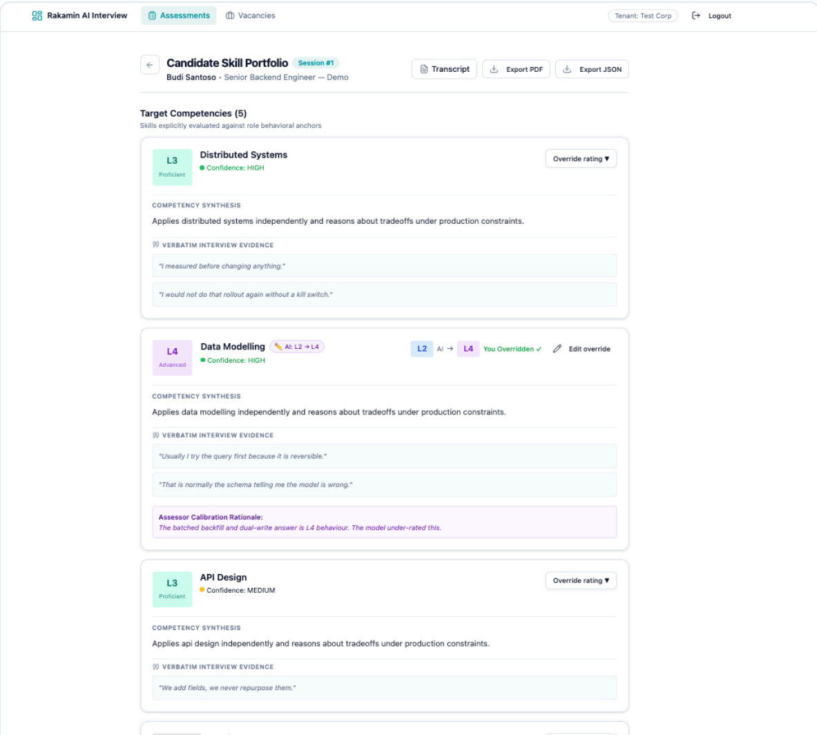
Figure 5.1 — Candidate Skill Portfolio: Multi-dimensional competency cards displaying proficiency badges (L1–L5), confidence indicators, expandable verbatim transcript quote accordions, and human assessor calibration banners.
