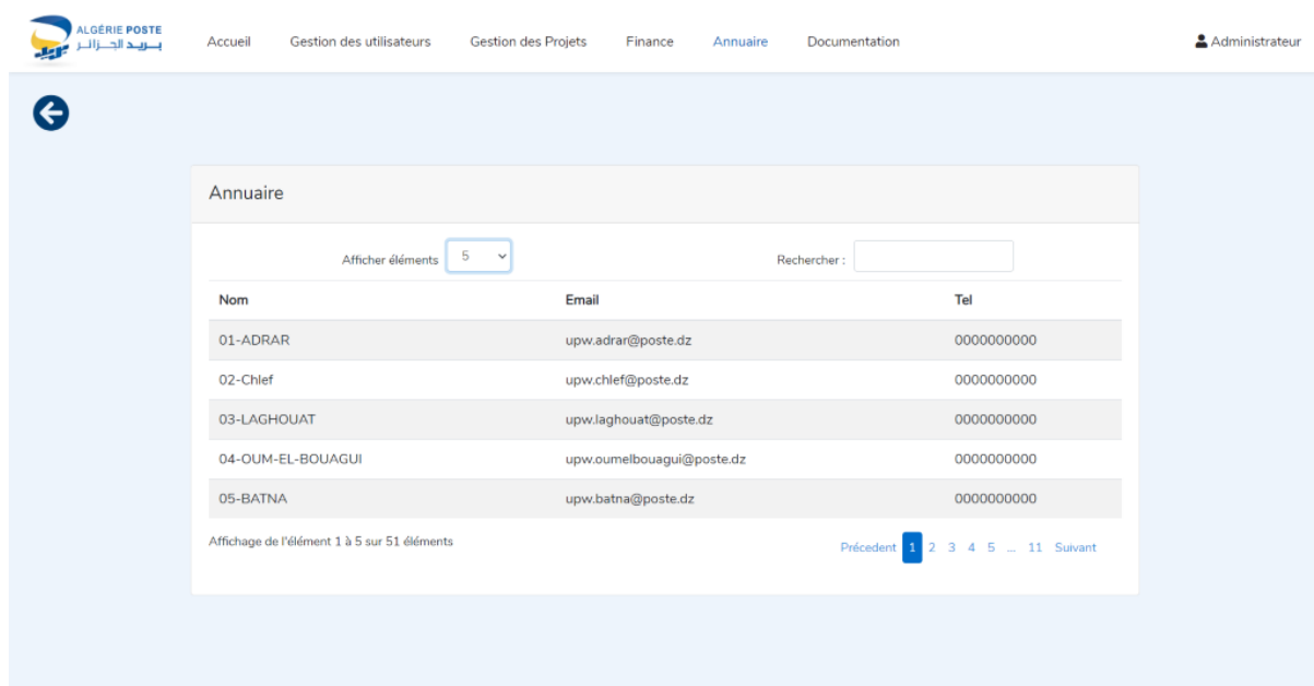
Figure 10. Annuaire.
