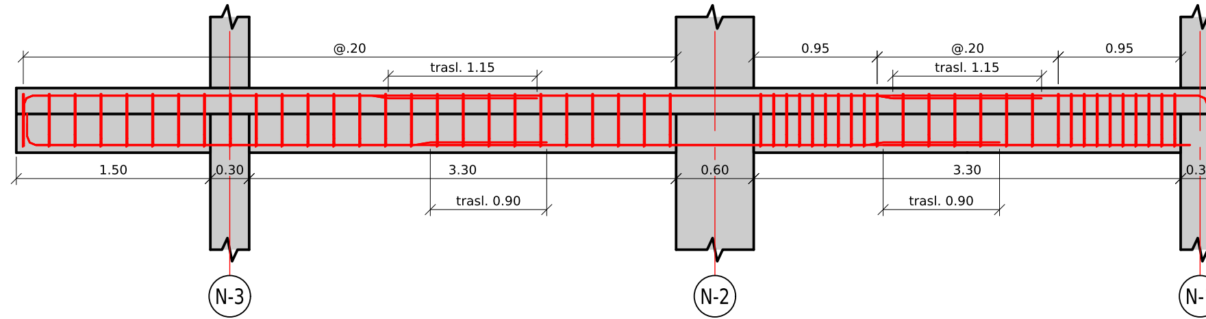
VIGA EJE A-4 (N2 a N5: sup. 5/3/3/3 Ø3/4", inf. 4 Ø3/4")
