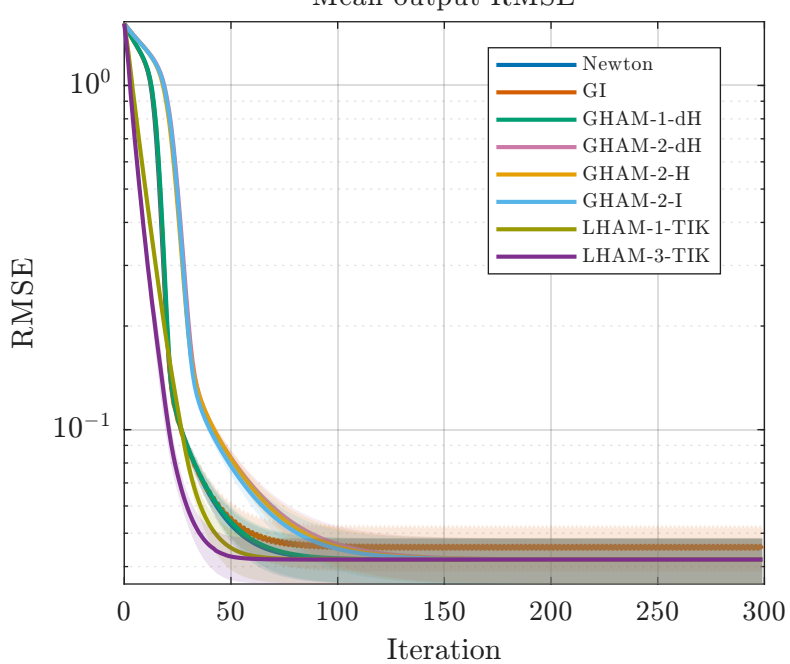
Mean output RMSE
