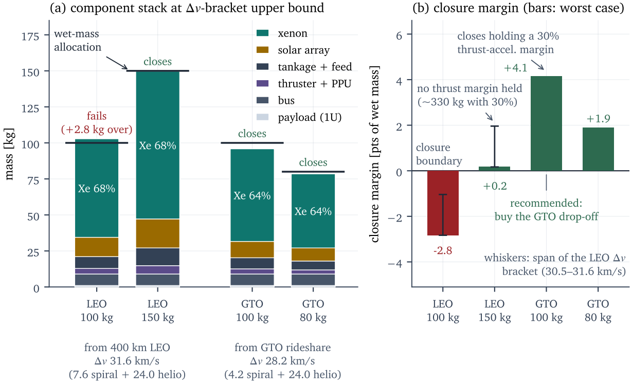
Figure 10. (a) Stacked component masses (payload, bus, thruster and power processing, tankage, solar array, xenon) at the conservative upper end of the heliocentric \Delta v reference interval; the horizontal cap on each bar marks the available wet mass. (b) Closure margin in percentage points of wet mass; whiskers span the reference \Delta v interval for the LEO cases. A 100 kg vehicle with a LEO start exceeds its cap everywhere in the interval; 150 kg closes, and both 100 kg and 80 kg close with a GTO start.
