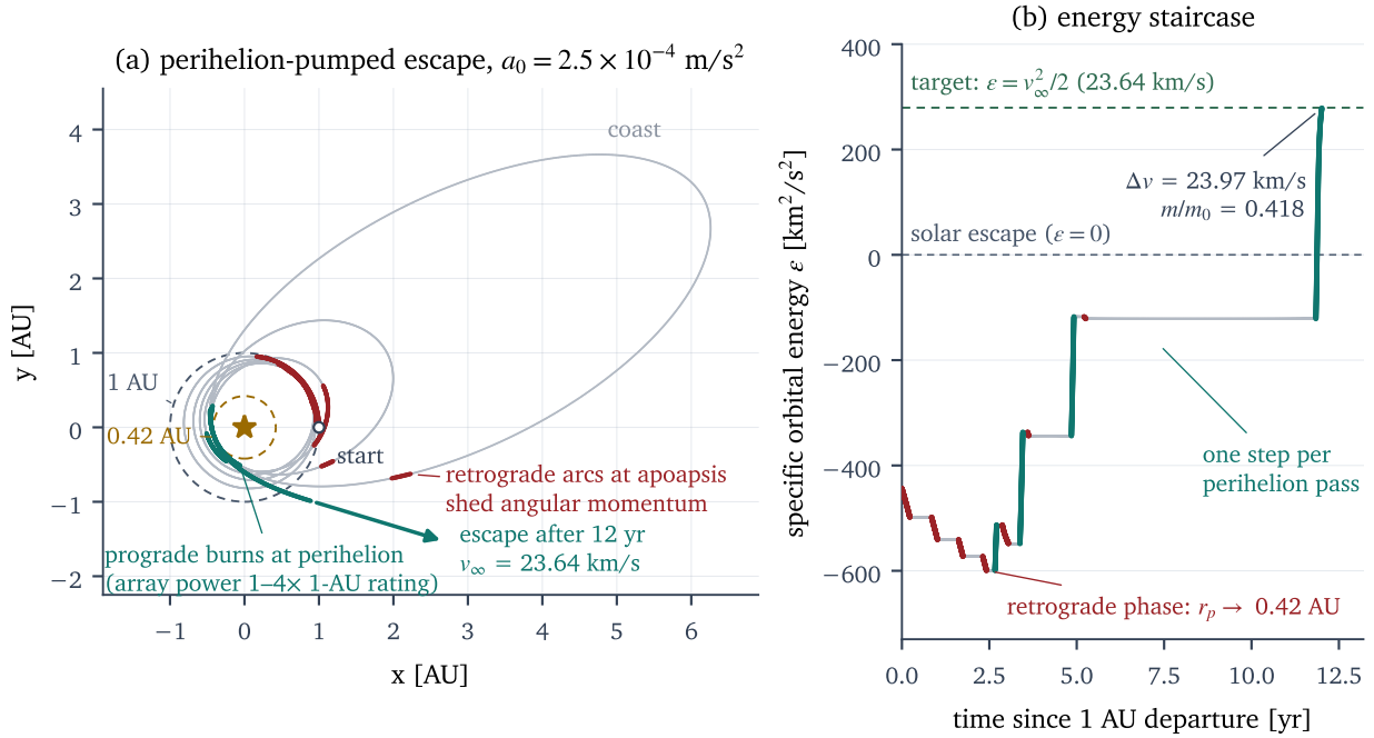
Figure 6. The optimized perihelion-pumping escape at a_0 = 2.5 \times 10^{-4} \text{ m s}^{-2} . (a) Heliocentric trajectory colored by thrust state (retrograde, coast, prograde), with the 1 AU and 0.42 AU circles dashed. Retrograde arcs near 1 AU lower perihelion to 0.42 AU, just inside the radius at which the thermal power cap of Equation 6 engages, so that array power at perihelion stands at one to four times its 1-AU rating. Prograde arcs then concentrate near perihelion, where power is highest and where, by the same Oberth logic that favors the perigee burn in the impulsive case, each increment of \Delta v buys the most orbital energy. Successive revolutions raise aphelion while the perihelion burns repeat, until the orbit reaches escape energy. In effect, the multi-revolution structure recovers for low thrust the perihelion-burn advantage that a single fast pass cannot provide at these thrust levels. (b) Specific orbital energy versus time, colored by thrust state: each prograde perihelion pass adds one step to the energy staircase; the vehicle reaches escape energy at 12.0 yr with \Delta v = 23.97 \text{ km s}^{-1} and final mass fraction 0.418.
