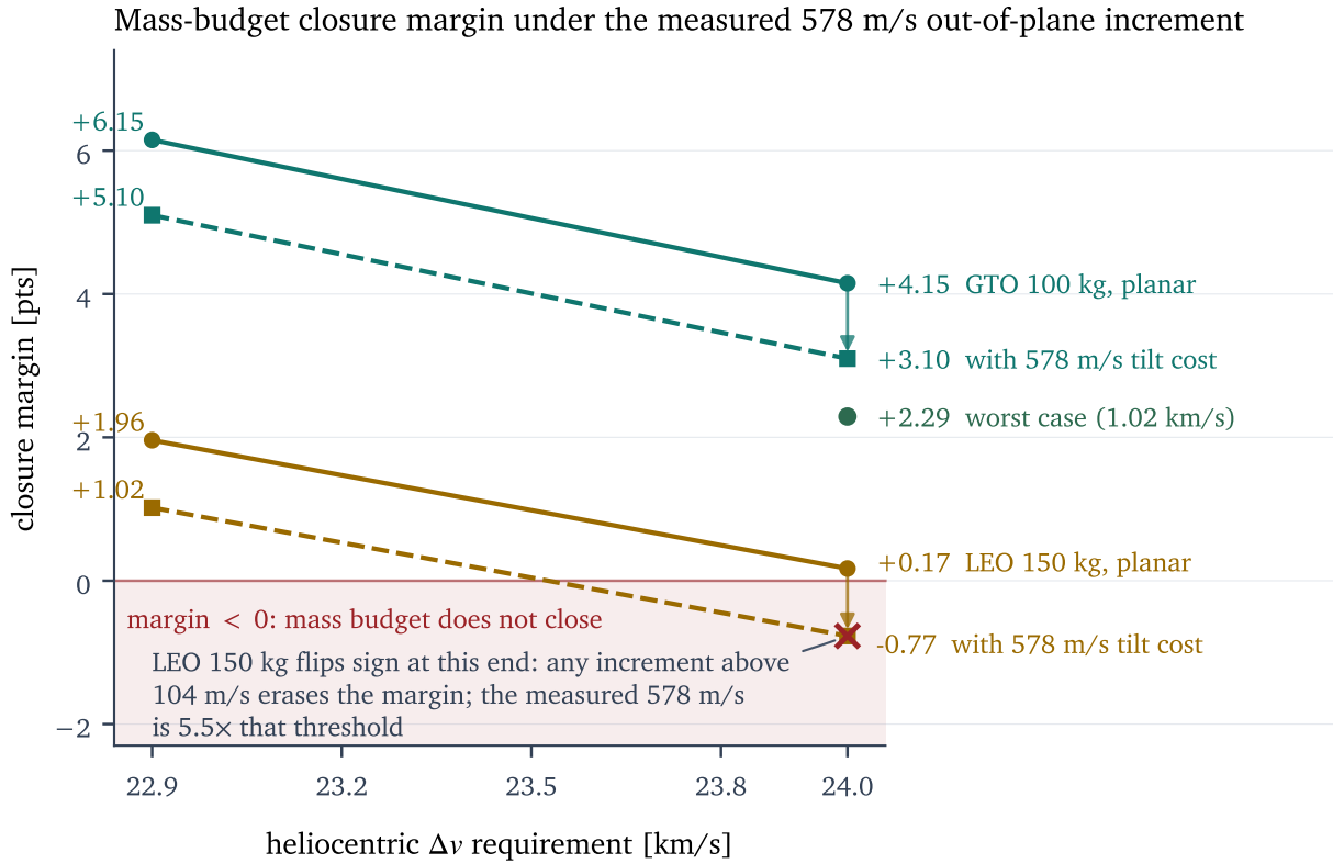
Figure 11. Closure margins re-evaluated with the measured 0.58 \text{ km s}^{-1} out-of-plane increment, in percentage points of wet mass at both ends of the heliocentric \Delta v reference interval. The 100 kg vehicle with a GTO start closes at both ends (+5.1 and +3.1 points, and +2.3 even at the planar band's 1.02 \text{ km s}^{-1} worst case); the 150 kg LEO fallback closes at the favorable end (+1.0) but fails at the conservative end (−0.8). Any increment above roughly 0.10 \text{ km s}^{-1} erases the conservative-end margin of the 150 kg LEO vehicle; the measured value is more than five times that threshold.
