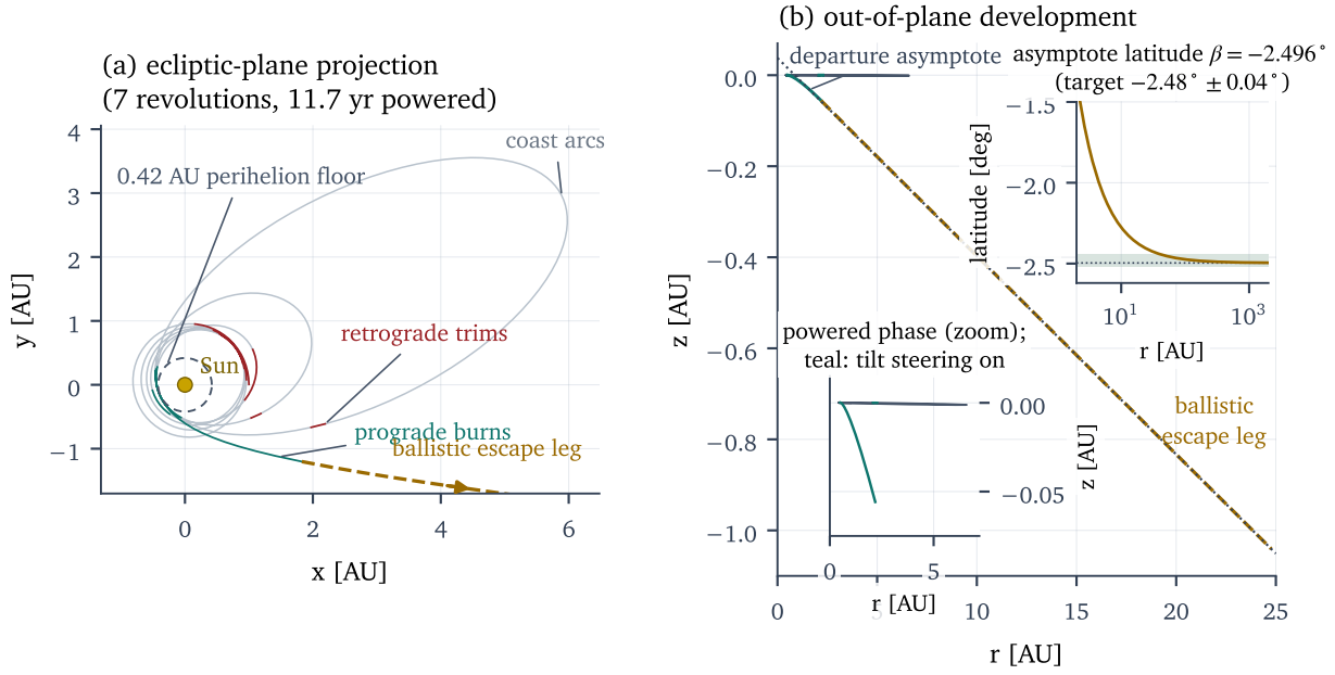
Figure 9. The three-dimensional perihelion-pumping escape at a_0 = 2.5 \times 10^{-4} \text{ m s}^{-2} , with the departure asymptote directed 2.48^\circ below the ecliptic (achieved within the 0.04^\circ aiming gate). Out-of-plane excursions stay below 0.06 AU and concentrate late in the escape, after the orbit is already hyperbolic. The measured cost of the tilt is 0.58 \text{ km s}^{-1} over the planar schedule, for a total of 24.56 \text{ km s}^{-1} .
