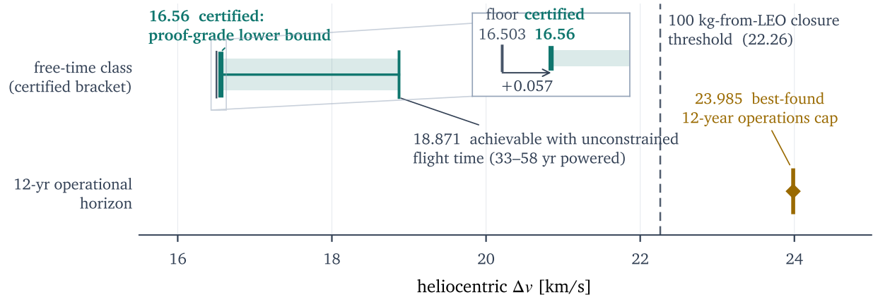
Figure 8. Two-class structure of the heliocentric \Delta v requirement. Upper row: with flight time unconstrained, the optimum lies between the certified lower bound of 16.56 \text{ km s}^{-1} and an integrated trajectory at 18.87 \text{ km s}^{-1} after about 58 years of powered flight (gate-passing schedules span 33–58 years at 18.9\text{--}20.5 \text{ km s}^{-1} ); the 16.50 \text{ km s}^{-1} bi-parabolic floor that the certified lower bound supersedes appears below the bracket. Lower row: on the 12-year operational horizon, the best schedule found costs 23.98 \text{ km s}^{-1} , a best-found value from a converged search; it does not bound the true optimum. The dashed line marks the 22.26 \text{ km s}^{-1} crossover below which a 100 kg vehicle from low Earth orbit would close. The unconstrained-flight-time trajectory lies below that crossover, so the concept fails on schedule; the trajectory class itself permits closure.
