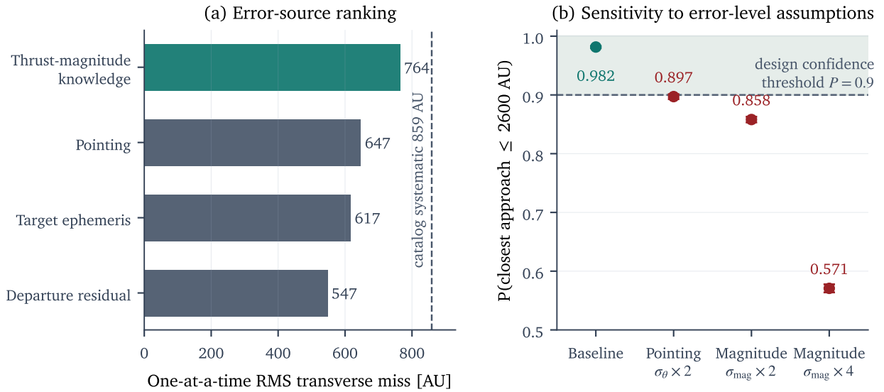
Figure 13. (a) Error-source ranking by one-at-a-time RMS transverse miss: thrust-magnitude knowledge (764 AU) leads pointing (647 AU), target ephemeris (617 AU), and the departure residual (547 AU), so thrust calibration is the highest-leverage mitigation. (b) Sensitivity of the success probability to the assumed error levels: the baseline 0.982 falls to 0.897 under a doubled pointing assumption, to 0.858 under a doubled thrust-magnitude assumption, and to 0.571 under a quadrupled one; each excursion falls below a 0.9 design confidence threshold. The verdict holds under the stated budget and fails under factor-of-two growth in either execution assumption.
