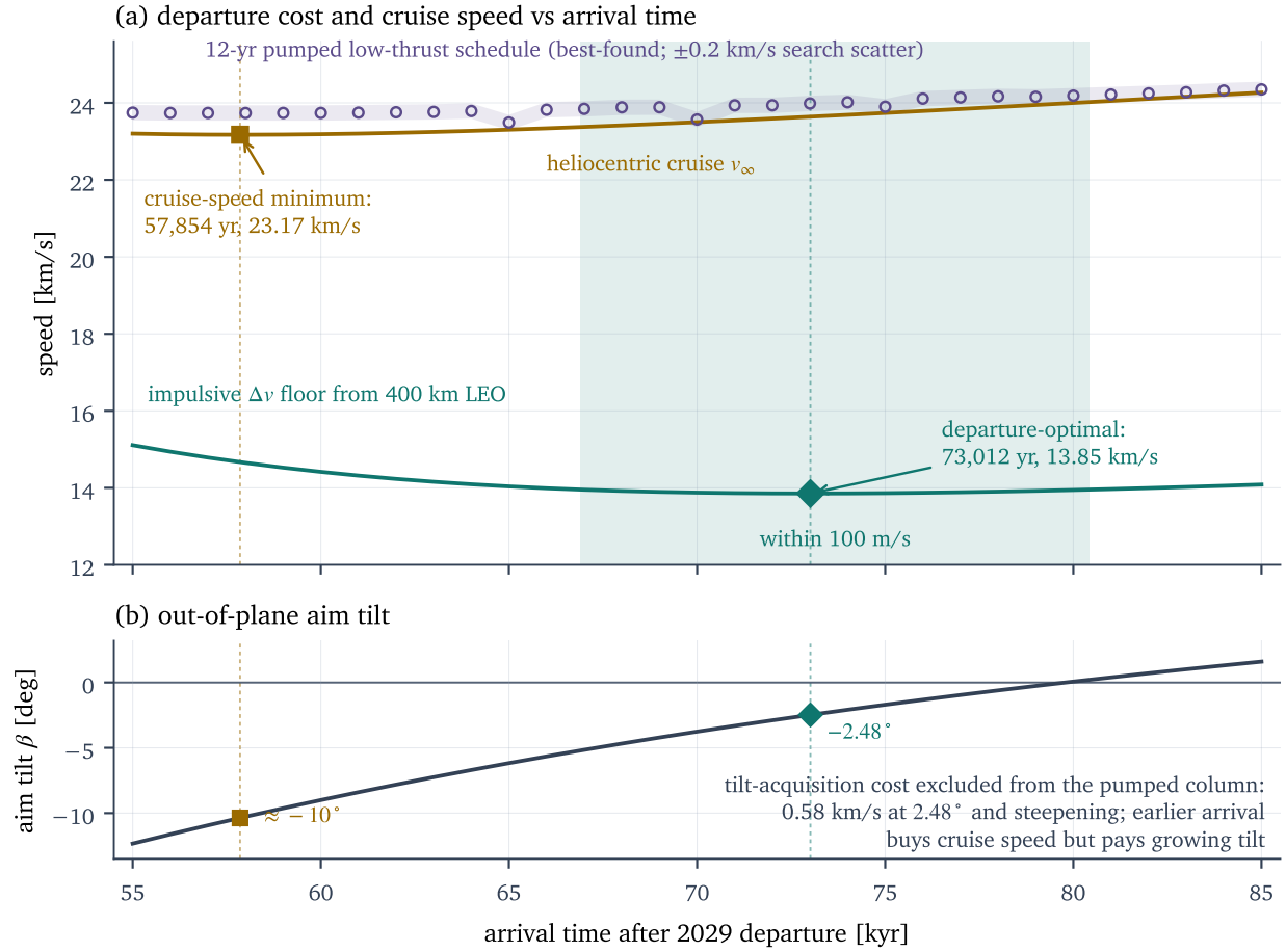
Figure 4. The arrival-epoch trade has two optima. (a) Impulsive departure floor from a 400 km low Earth orbit, required cruise v_\infty , and the best 12-year pumping schedule found at each arrival epoch (open circles; each an upper bound on its optimum, with roughly \pm 0.2 km s ^{-1} scatter between search seeds). The departure- \Delta v optimum falls at 73,012 years and stays within 100 m s ^{-1} across the shaded 66,908–80,436-year basin; the cruise-speed minimum falls at 57,854 years, 23.17 km s ^{-1} . (b) Aim tilt \beta versus arrival epoch: the tilt steepens from -2.48^\circ at the departure- \Delta v optimum to about -10^\circ near the cruise-speed minimum, and the cost of acquiring the tilt (0.58 km s ^{-1} at 2.48^\circ ; excluded from the pumping-schedule column) grows with it. Earlier arrival buys cruise speed but pays growing tilt.
