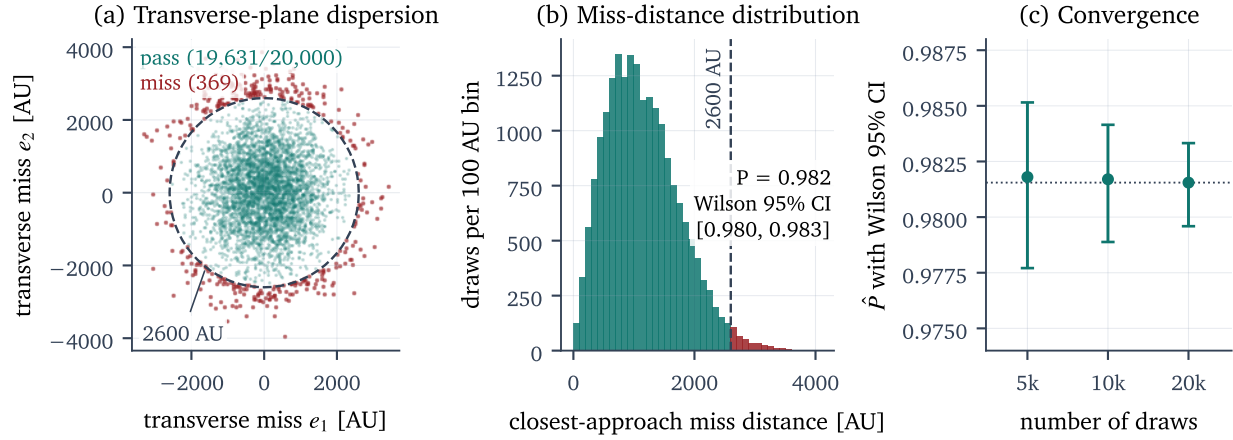
Figure 12. Encounter dispersion under the combined error budget, from the 20,000-draw seeded Monte Carlo. (a) Dispersion in the plane transverse to the approach velocity: 19,631 of 20,000 draws (teal) fall inside the 2600 AU requirement circle, 369 (red) outside. (b) Distribution of closest-approach miss distance against the requirement: the median miss is 1076 AU, the 97.5th percentile 2499 AU, and P = 0.982 of draws pass inside the sphere (95% confidence interval [0.980, 0.983]). (c) Convergence: the estimate is stable across the first 5,000, 10,000, and full 20,000 draws, with the confidence interval narrowing as 1/\sqrt{n} . An independent analytic error-propagation model, sharing no code or random draws with the simulation, reproduces the success probability to 0.011%.
