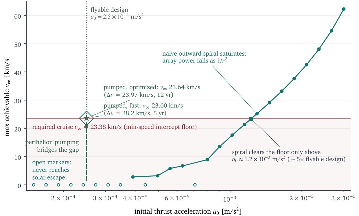
Figure 5. Achievable cruise speed versus initial thrust acceleration a_0 (logarithmic axis) for a conventional outward low-thrust spiral. The curve saturates below the 23.38 \text{ km s}^{-1} cruise floor (horizontal line) at every flyable thrust level and clears it only above a_0 \approx 1.2 \times 10^{-3} \text{ m s}^{-2} , roughly five times the design value. The two points above the line come from perihelion-pumping schedules at a_0 = 2.5 \times 10^{-4} \text{ m s}^{-2} : the saturation bounds outward spirals; it does not bound solar-electric propulsion as such.
