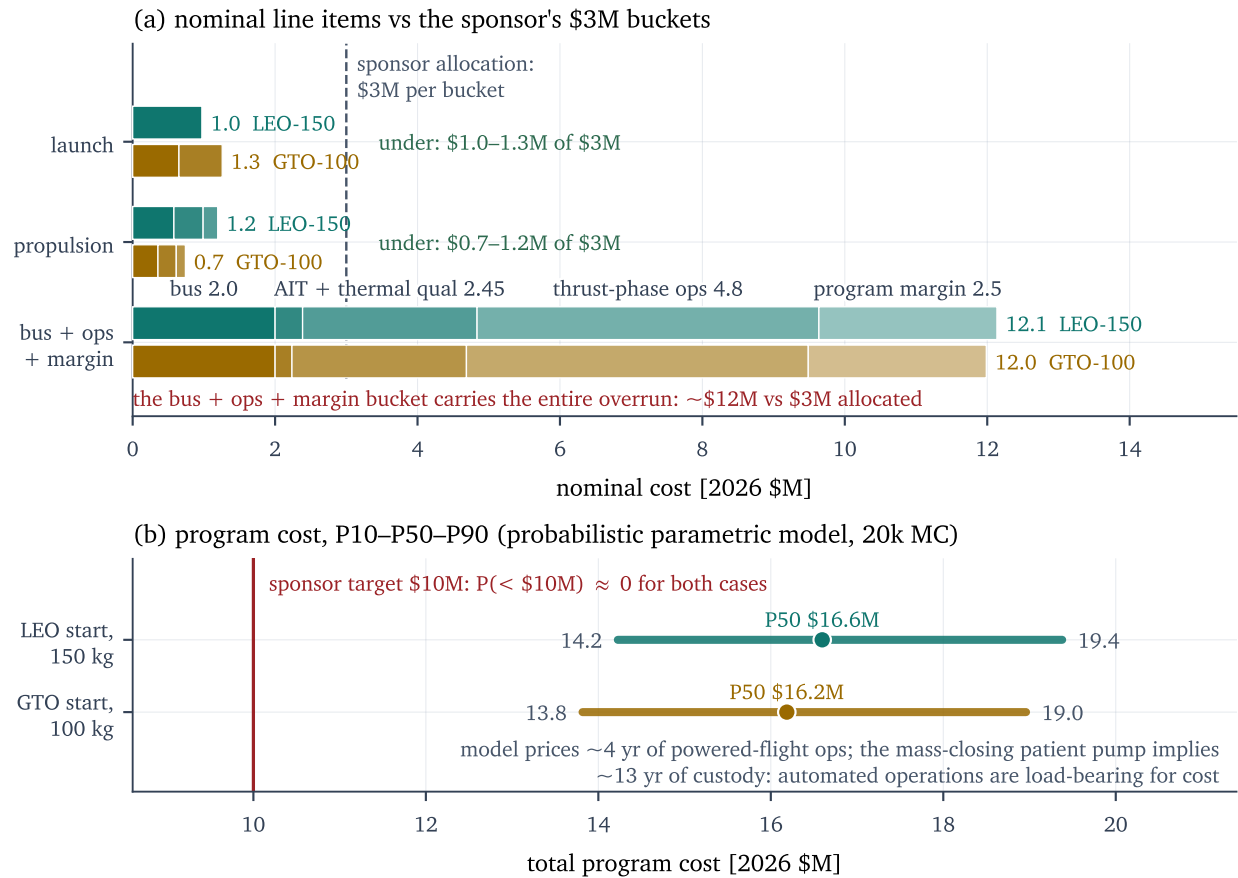
Figure 14. (a) Nominal cost by mission budget category for the two primary architectures, compared with the $3M/$3M/$3M allocation: launch and propulsion come in at roughly one third of their allocations, while the bus-and-operations category absorbs the entire overrun. (b) 10th–50th–90th-percentile total-cost ranges from the 20,000-draw Monte Carlo, compared with the $10M program target: no architecture's 10th percentile reaches the target.
