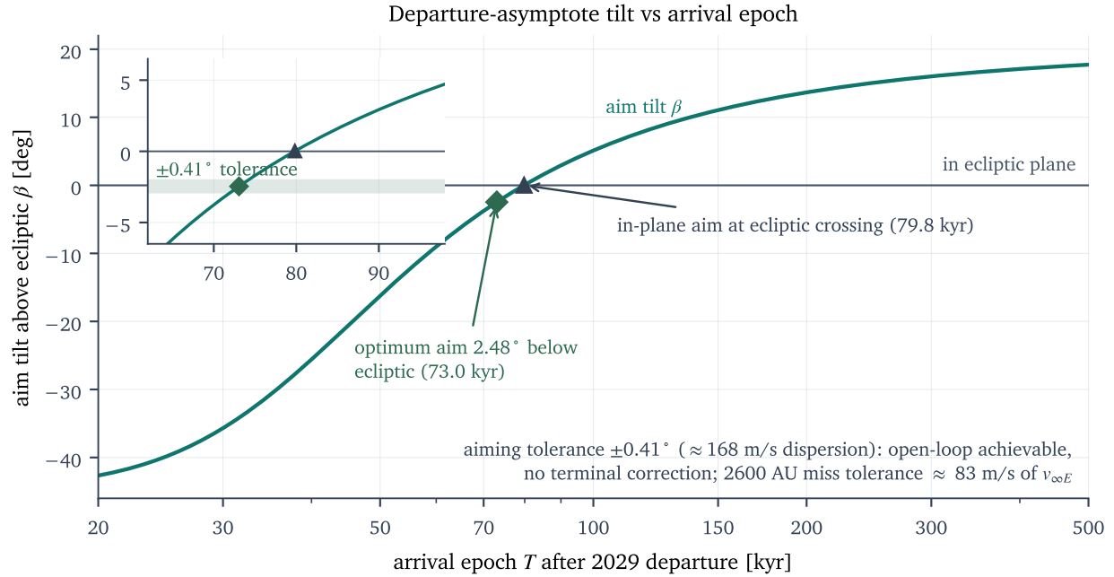
Figure 3. Departure aim tilt \beta versus arrival epoch; the inset shows the \pm 0.41^\circ open-loop aiming tolerance band around the optimum. The vehicle borrows Earth’s orbital velocity of 29.78 \text{ km s}^{-1} in plane only, so the tilt directly prices the out-of-plane component of the departure asymptote. The tilt passes through zero at the ecliptic-plane crossing (79,786 yr); the joint optimum accepts a 2.48^\circ tilt to intercept the star several thousand years earlier, when it is closer and slower to chase.
