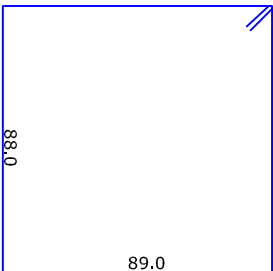
7xN2Ø10.0 C=374.0 374.0
