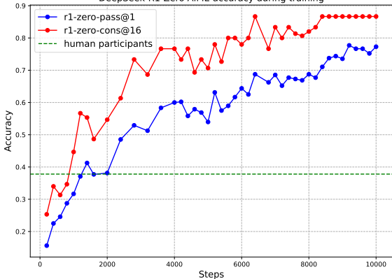
DeepSeek-R1-Zero AIME accuracy during training
