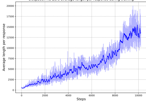
DeepSeek-R1-Zero average length per response during training
