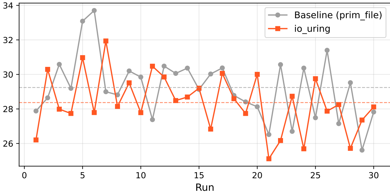
Confirm p99 latency (ms)
