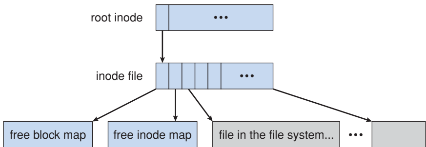
Figure 11.16 The WAFL file layout.
