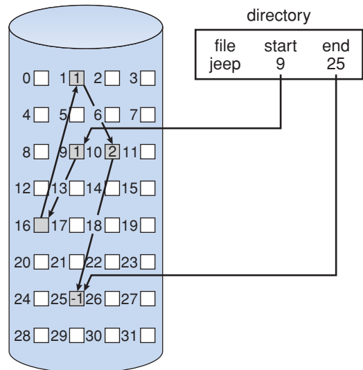
Figure 11.6 Linked allocation of disk space.
