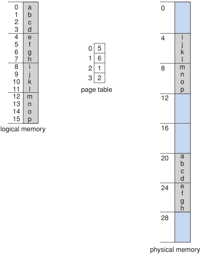
Figure 7.12 Paging example for a 32-byte memory with 4-byte pages.
