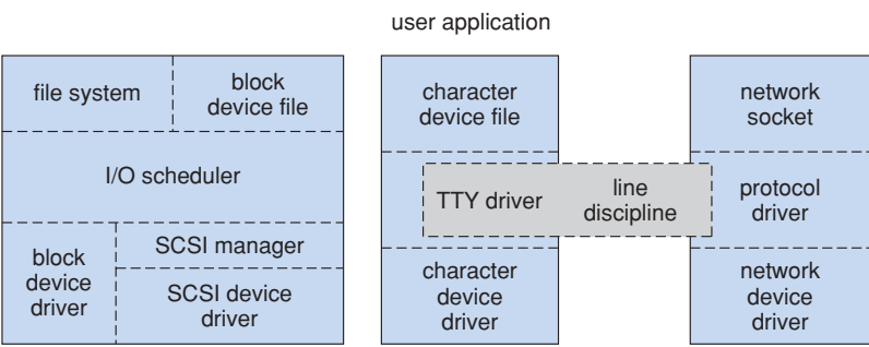
Figure 15.8 Device-driver block structure.
