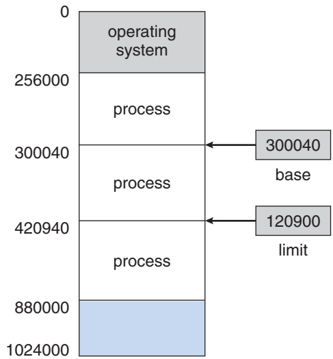
Figure 7.1 A base and a limit register define a logical address space.
