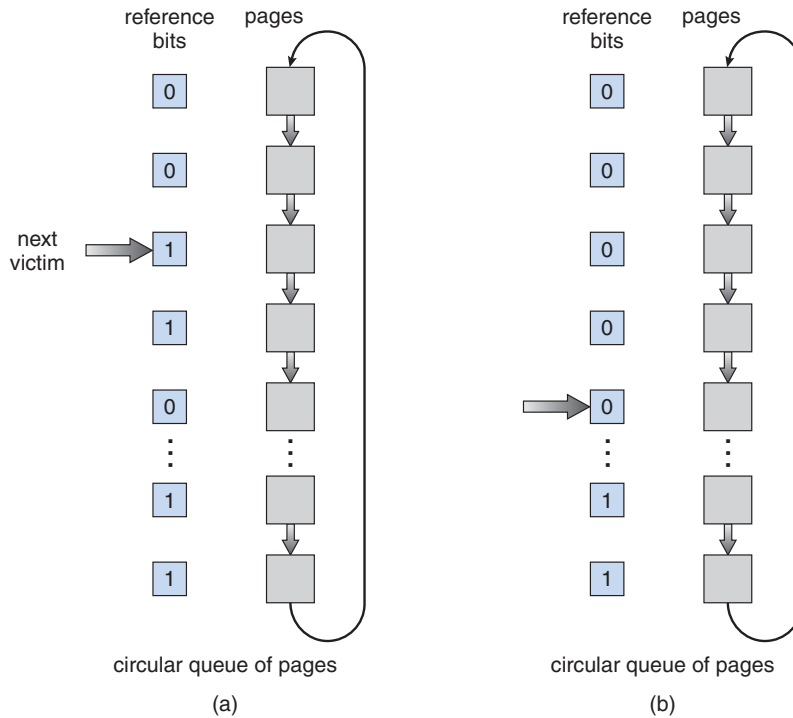
Figure 8.17 Second-chance (clock) page-replacement algorithm.
