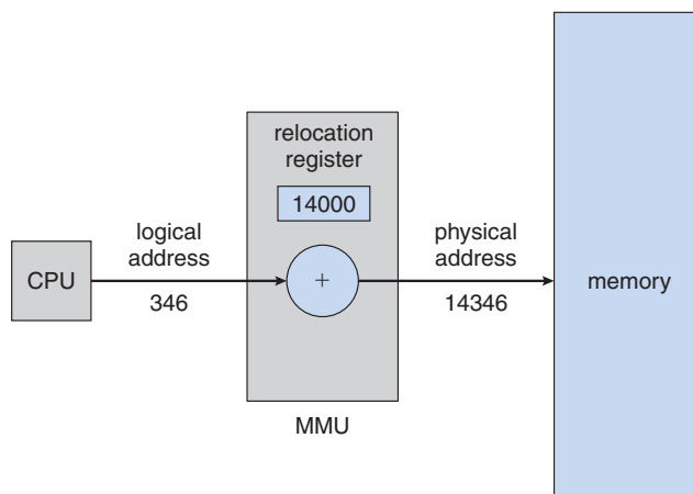
Figure 7.4 Dynamic relocation using a relocation register.
