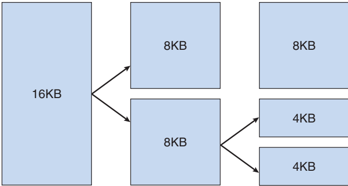
Figure 15.4 Splitting of memory in the buddy system.
