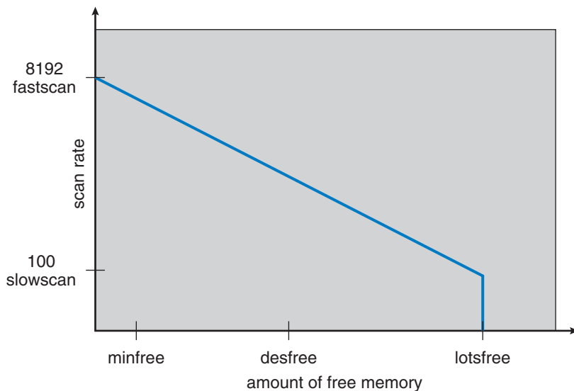
Figure 8.29 Solaris page scanner.
