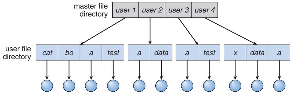
Figure 10.10 Two-level directory structure.
