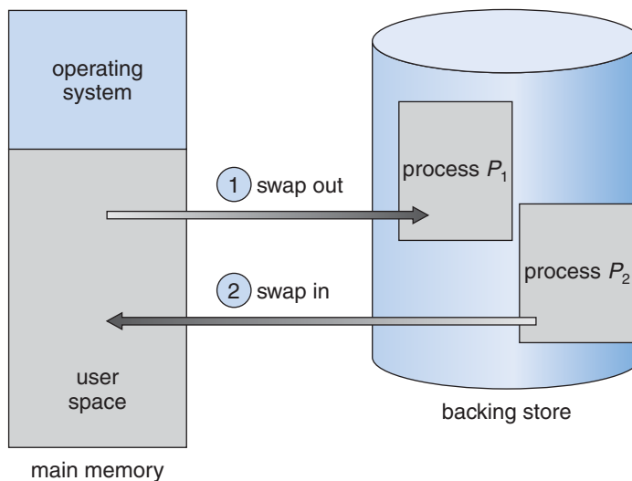
Figure 7.5 Swapping of two processes using a disk as a backing store.
