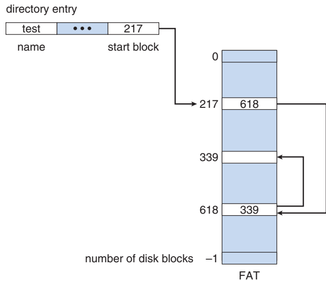
Figure 11.7 File-allocation table.
