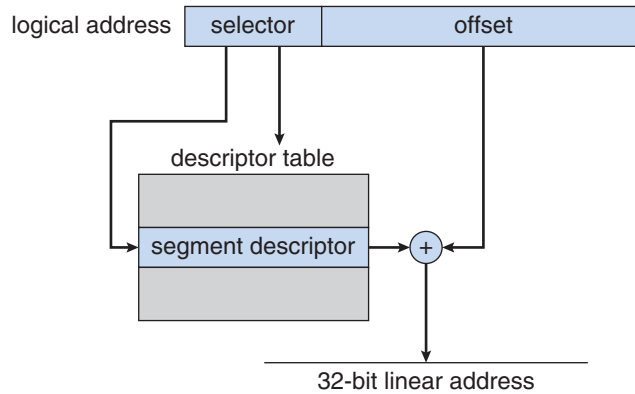
Figure 7.22 IA-32 segmentation.
