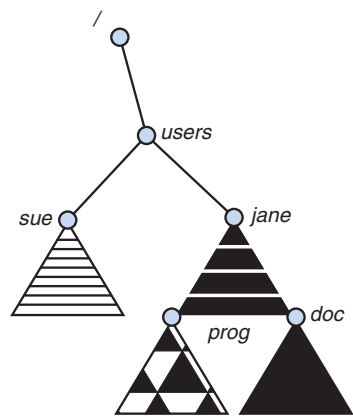
Figure 10.15 Mount point.
