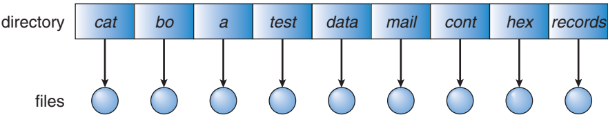
Figure 10.9 Single-level directory.
