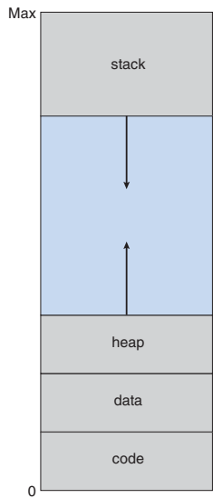
Figure 8.2 Virtual address space.
