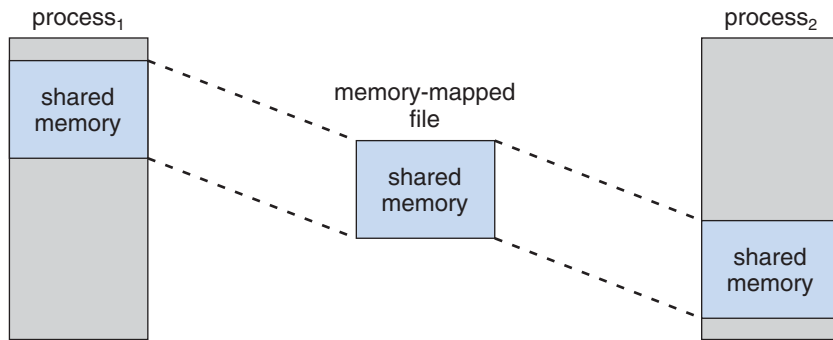
Figure 8.23 Shared memory using memory-mapped I/O.
