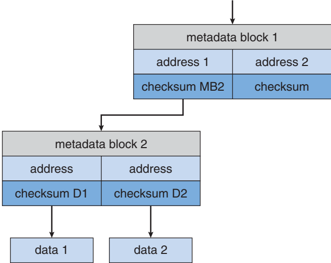
Figure 9.13 ZFS checksums all metadata and data.
