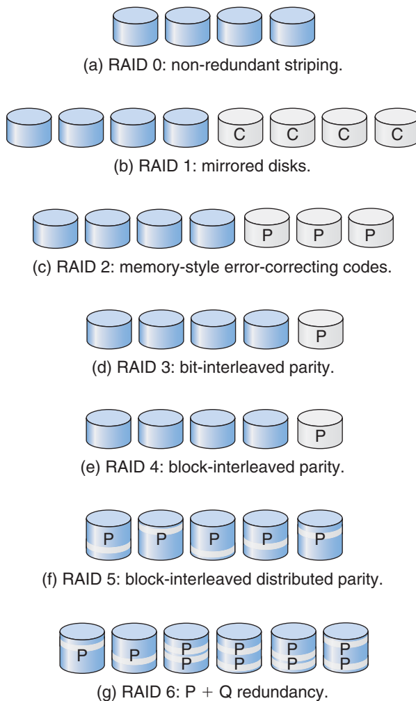
Figure 9.11 RAID levels.
