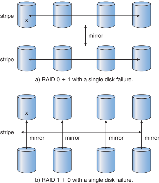
Figure 9.12 RAID 0 + 1 and 1 + 0.
