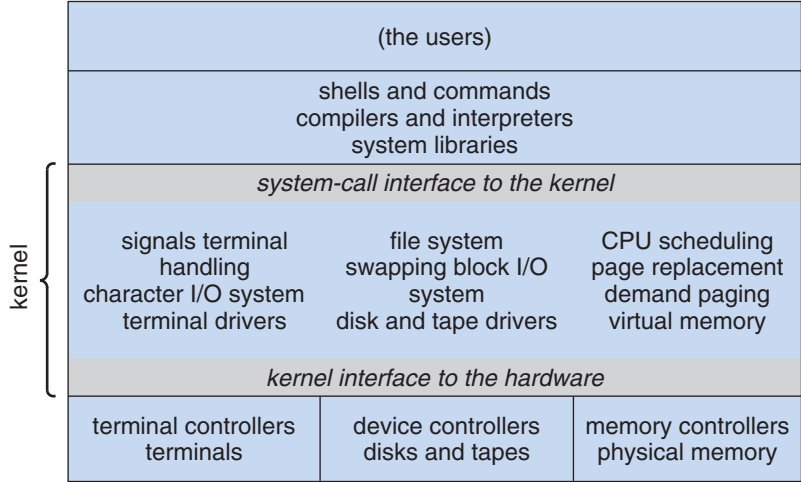
Figure 2.12 Traditional UNIX system structure.
