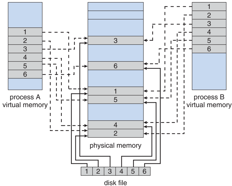
Figure 8.22 Memory-mapped files.
