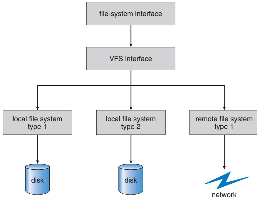
Figure 11.4 Schematic view of a virtual file system.
