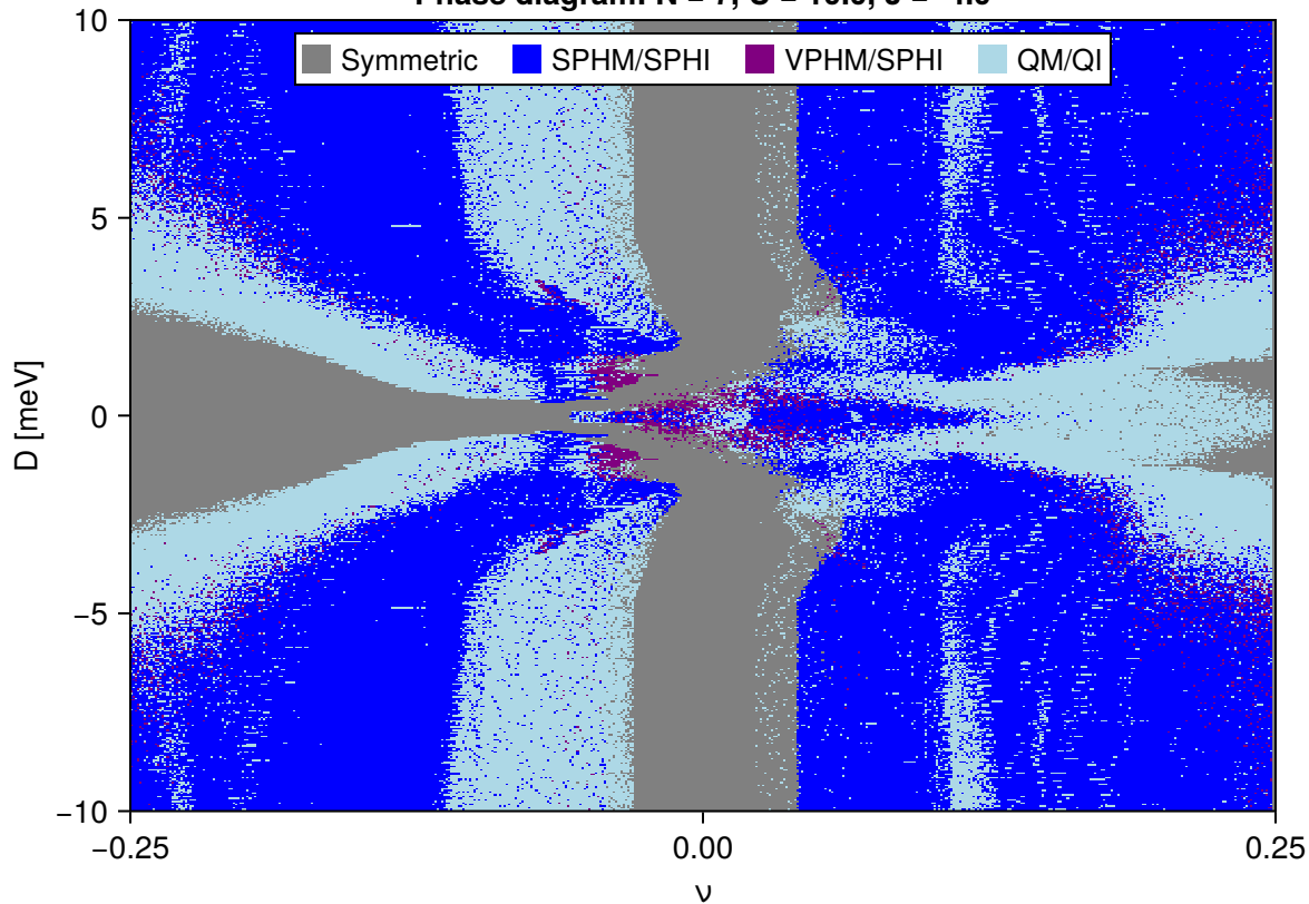
Phase diagram: N = 7 , U = 10.0 , J = -4.0
