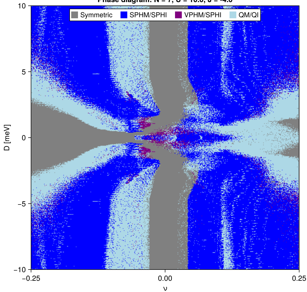
Phase diagram: N = 7 , U = 10.0 , J = -4.0
