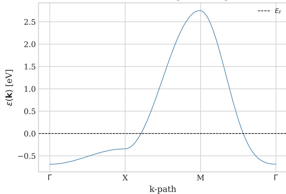
Hg-1212 — square-lattice tight-binding [APPROXIMATE] Band structure (tight-binding)
