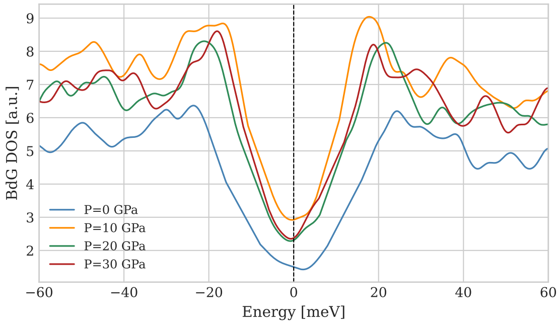
BdG density of states — d-wave gap \Delta_d = local pairing proxy (BdG); NOT T_{c\_zero}
