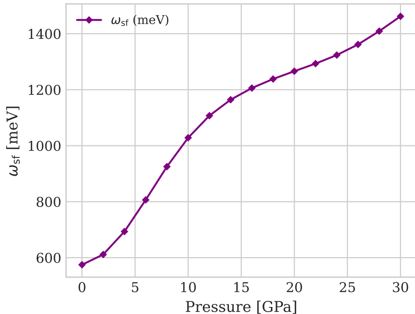
Paramagnon energy scale
