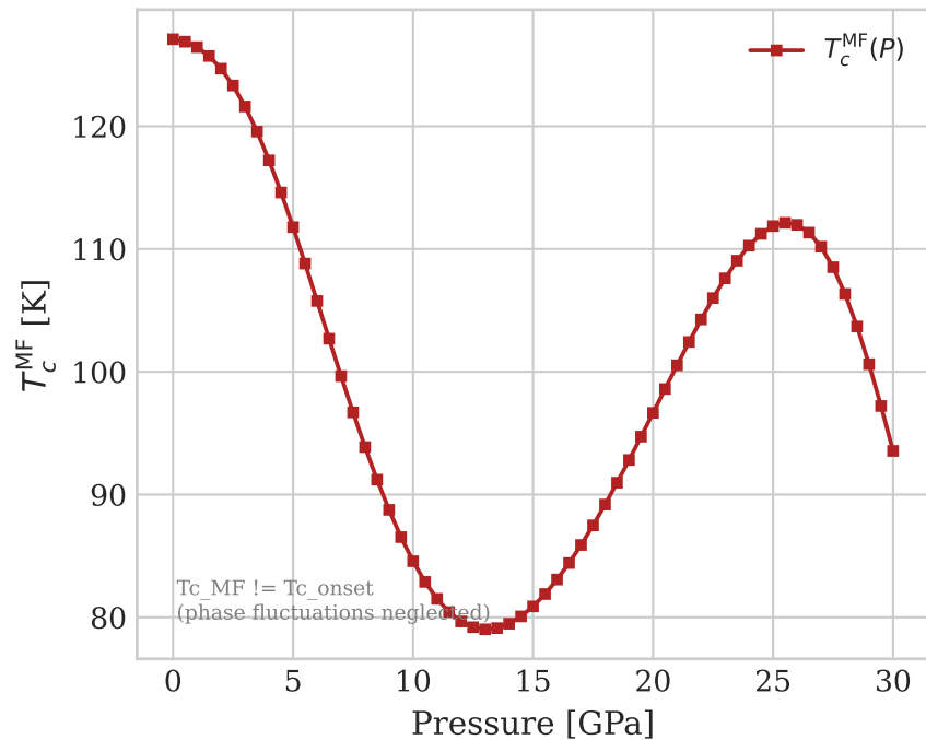
Mean-field T_c (BdG)
