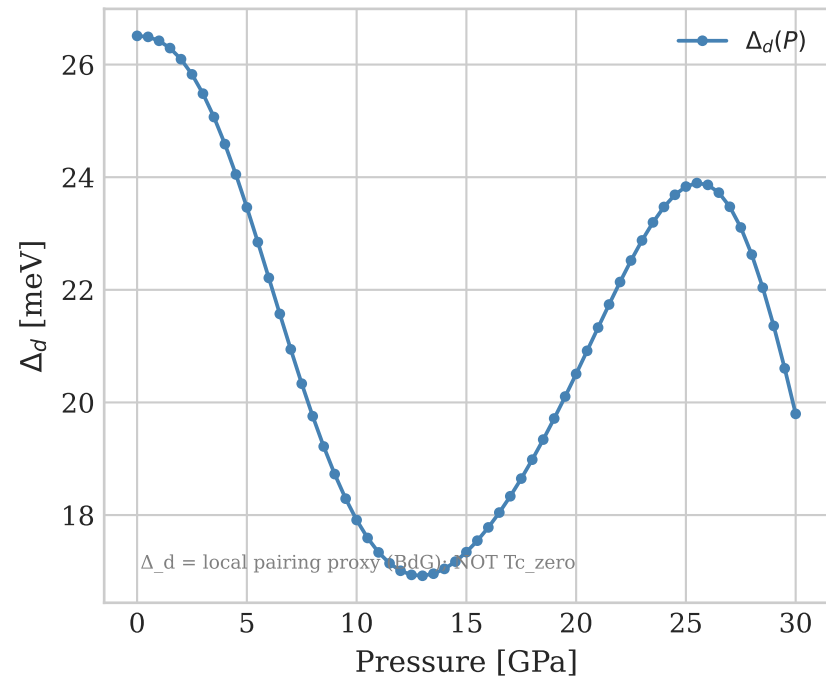
d-wave gap \Delta_d(P)
