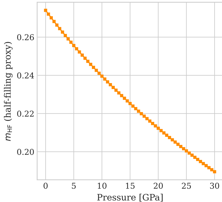
HF proxy magnetisation [LABEL B]
