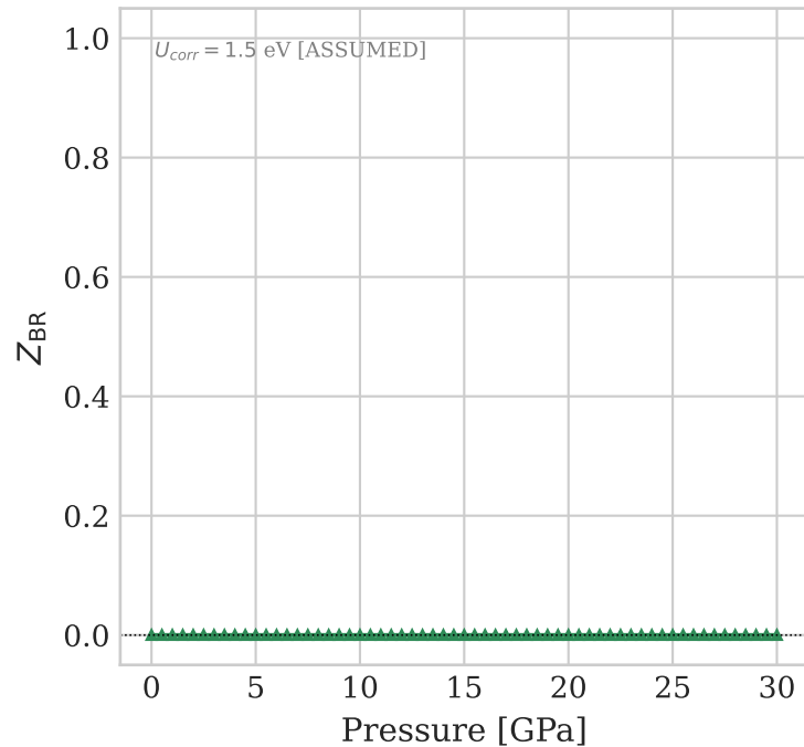
Brinkman-Rice Z [LABEL C]
