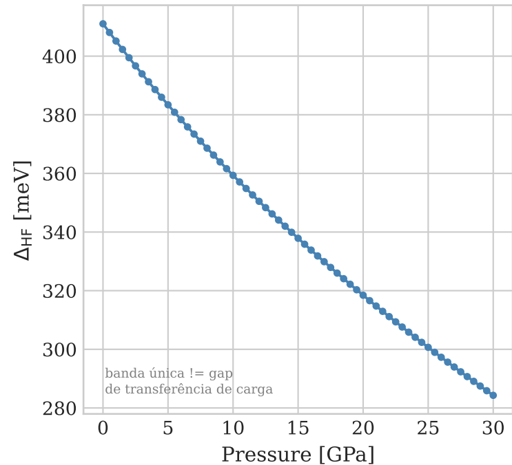
Hubbard-HF gap [LABEL A]
