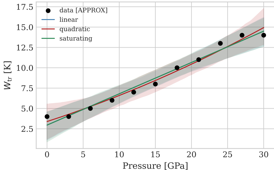
Null models — W_{\text{tr}} (shading = 95% bootstrap CI)
