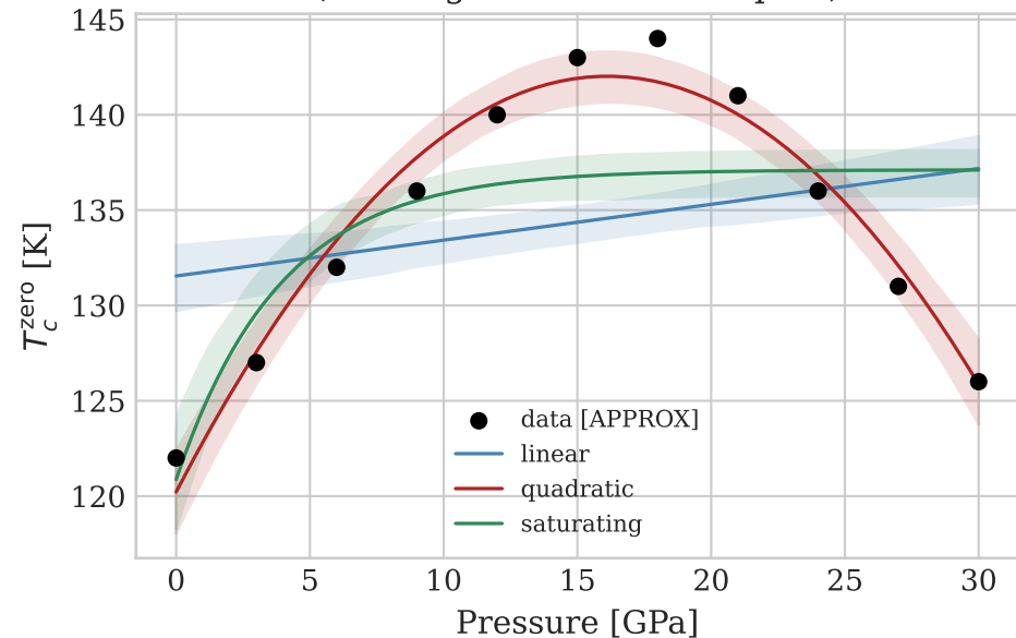
Null models — T_c _zero (shading = 95% bootstrap CI)
