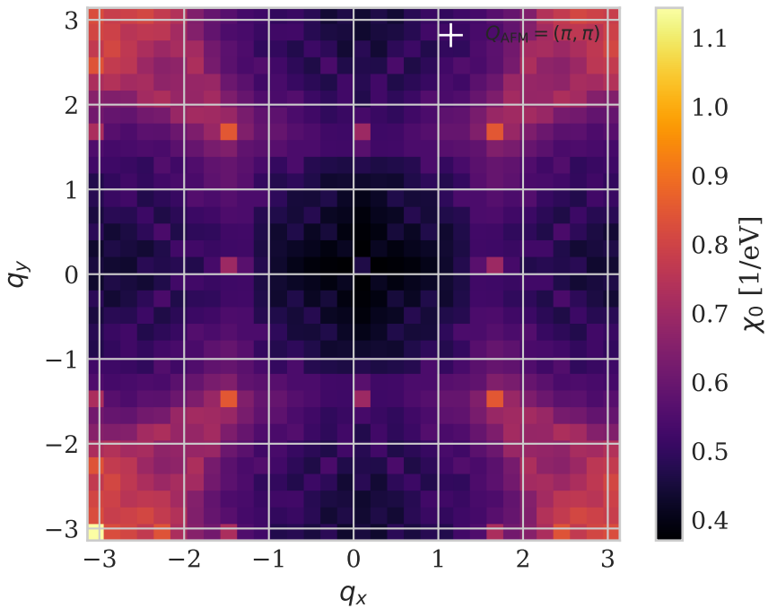
Static Lindhard \chi_0(\mathbf{q}) [P=0]
