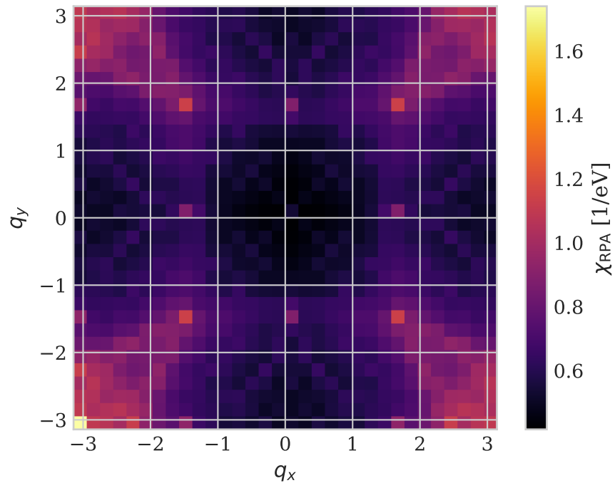
RPA susceptibility \chi_{\text{RPA}}(\mathbf{q}) [P=0]
