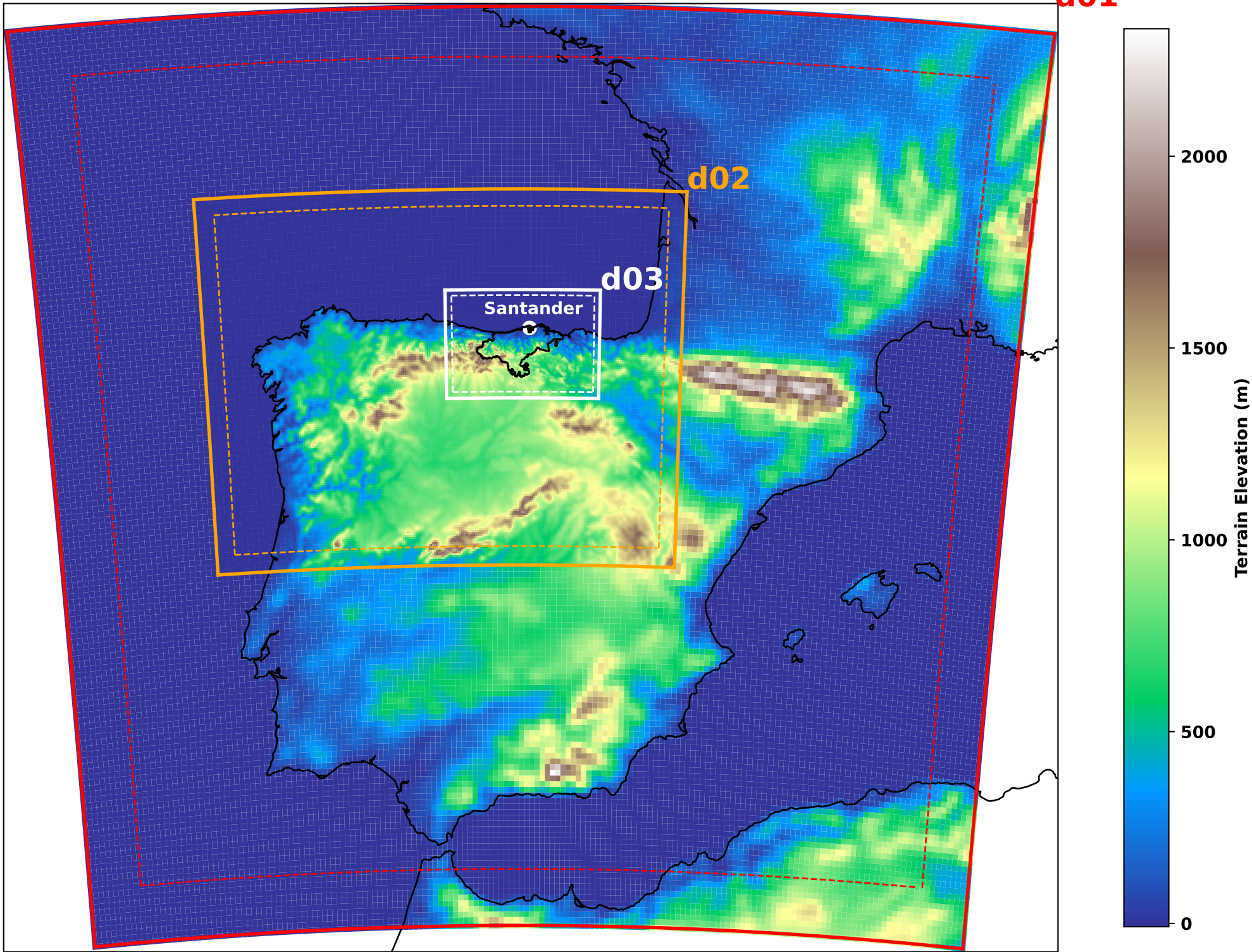
WRF Domains with Multi-Resolution Terrain, Relaxation Zones & Cantabria
