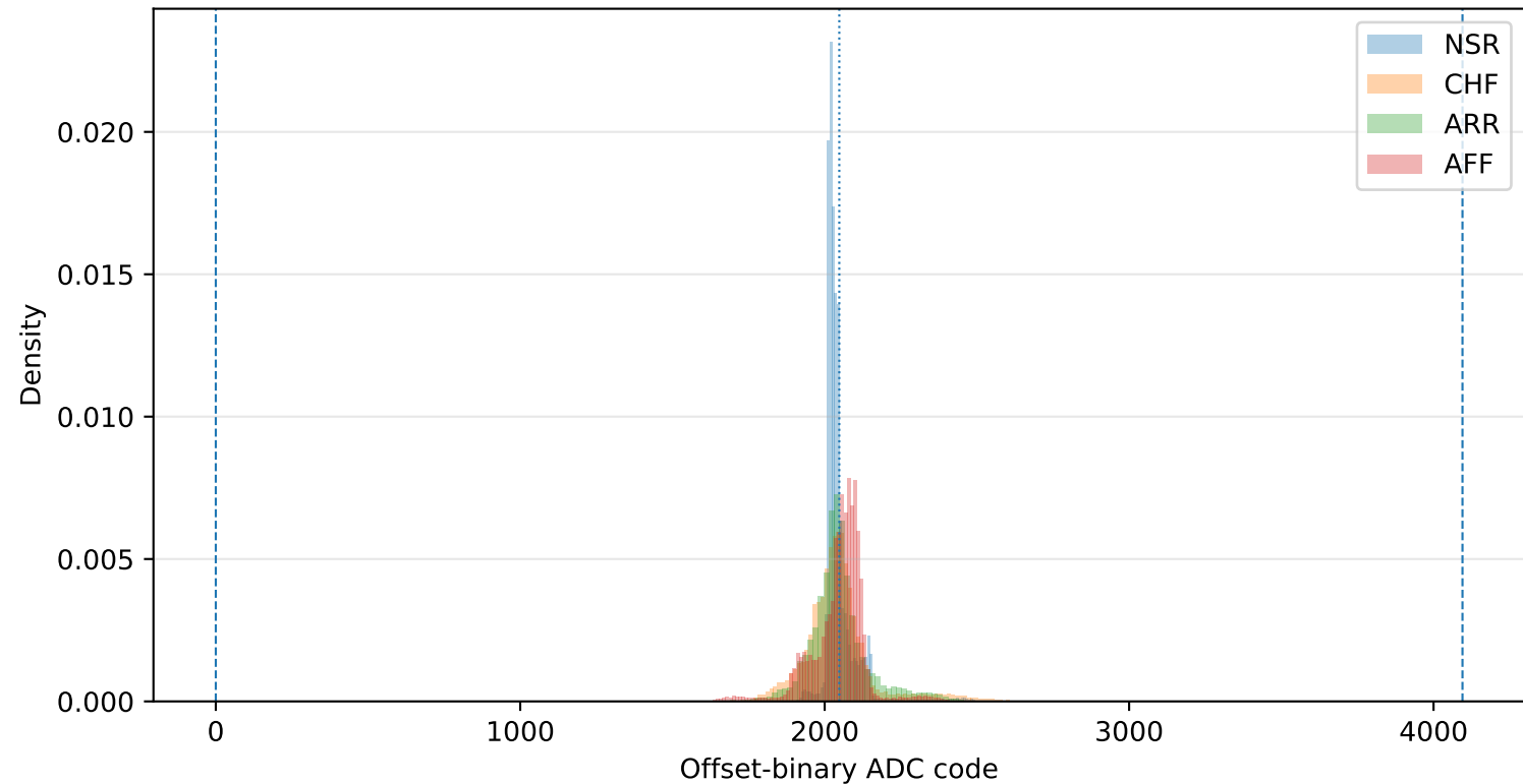
ADC Code Distribution Reference
