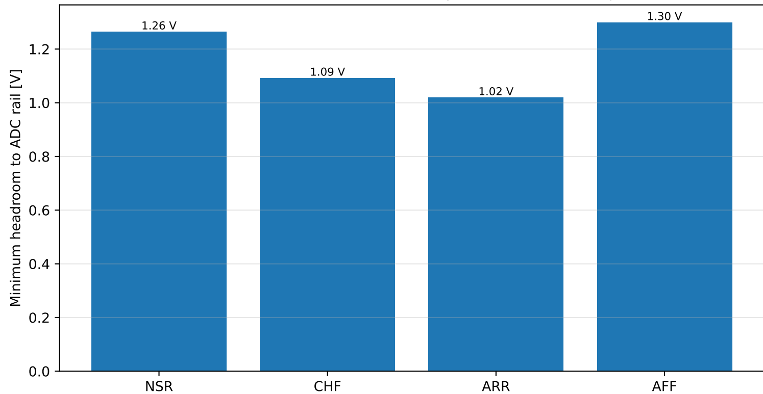
ADC Headroom Reference for Representative ECG Inputs
