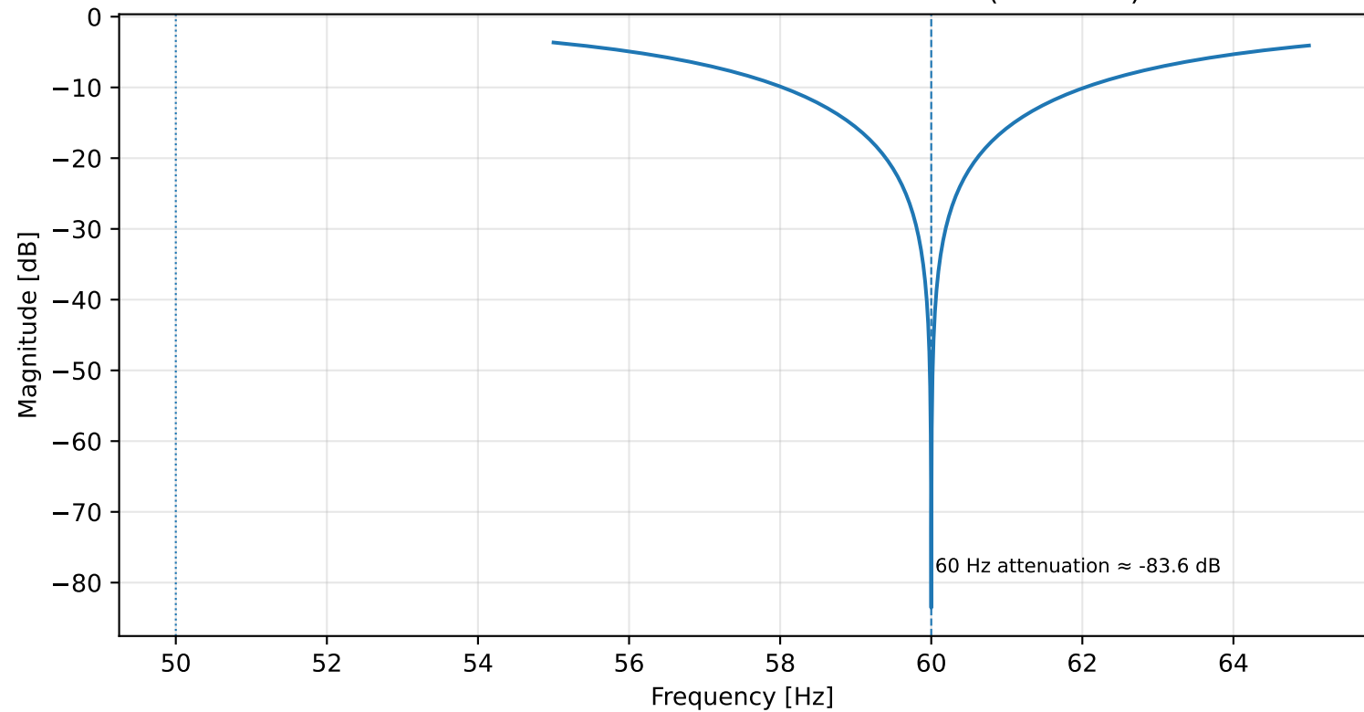
Dense 60 Hz Active Twin-T Notch Reference (55-65 Hz)
