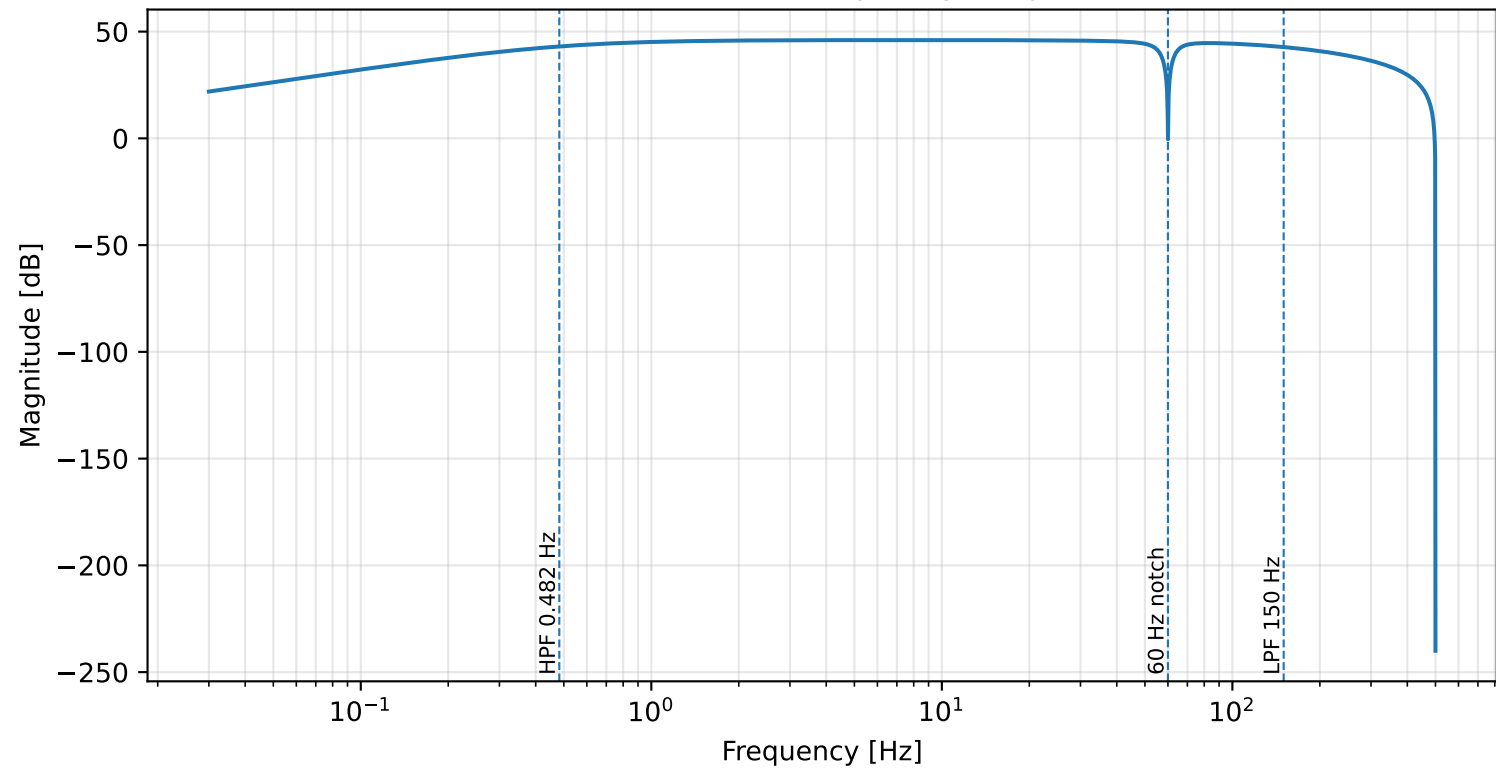
MATLAB Nominal AFE+ADC Frequency Response Reference
