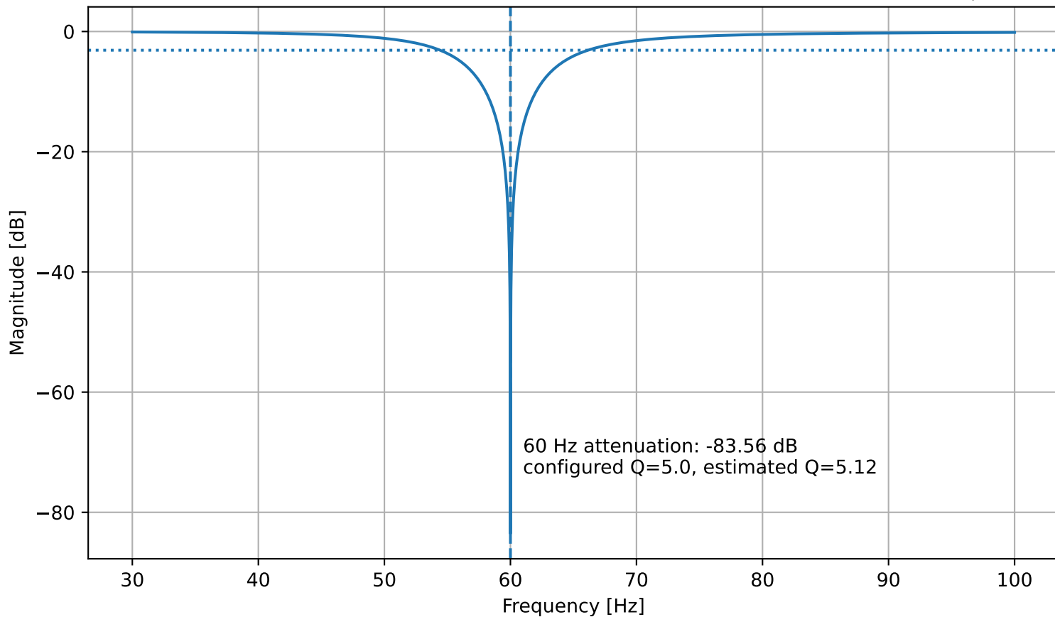
MATLAB Nominal Active Twin-T 60 Hz Notch Reference (30-100 Hz Sweep)
