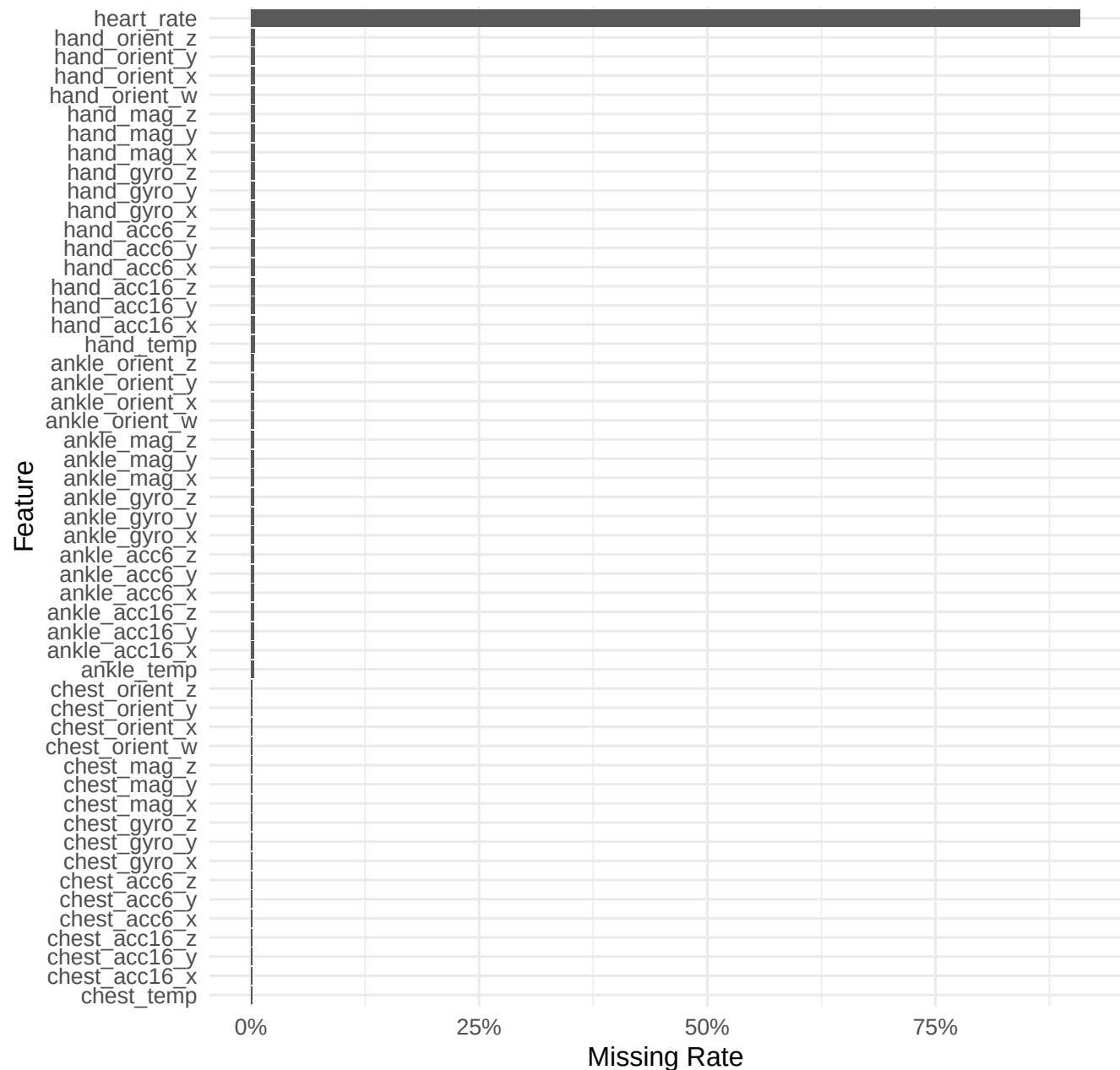
Missingness by Feature (Raw Data)
