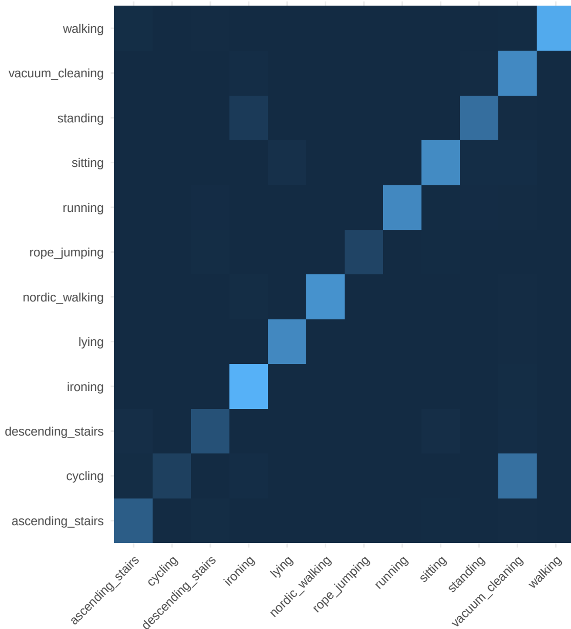
Final Confusion Matrix TEST (Subject-independent)
