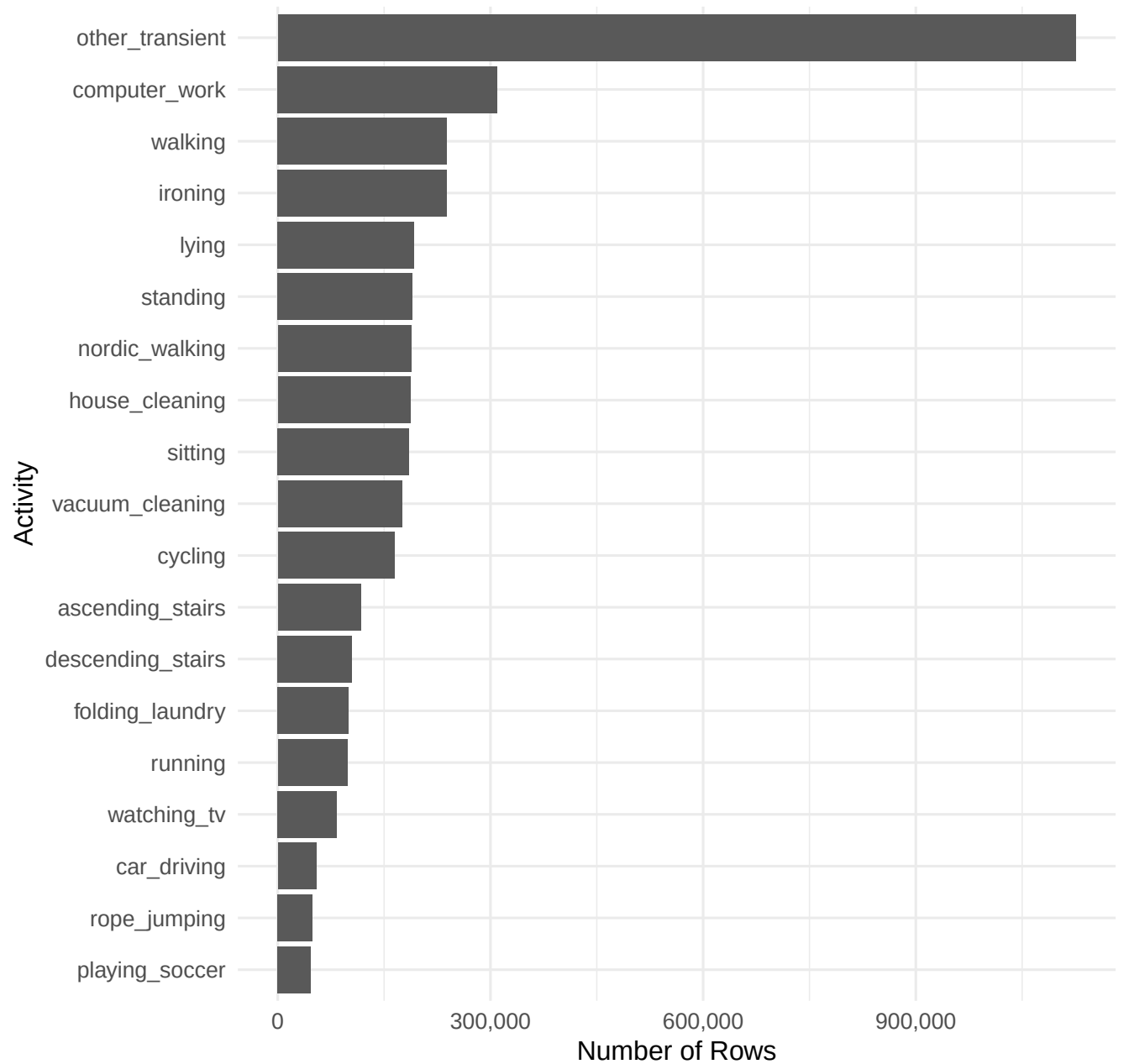
Activity Distribution (Raw Rows)
