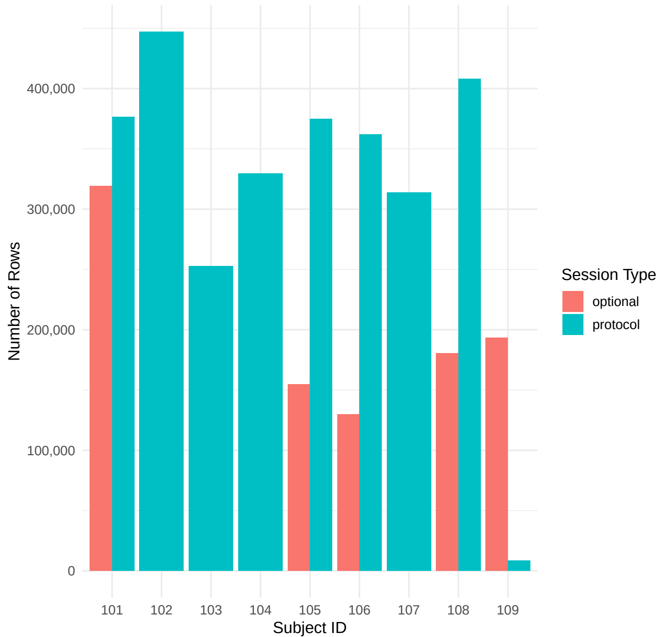
PAMAP2 Raw Data Coverage by Subject and Session Type
