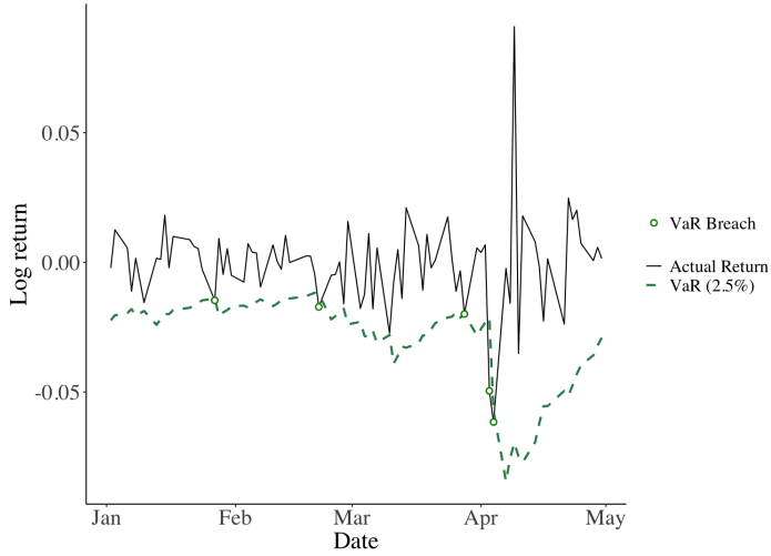
Figure 4.4: 2.5% VaR forecast and breaches in the test period, GJR-Asyt (5 breaches observed; 2 expected).
