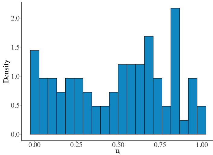
Figure 4.7: Histogram of PIT values, GARCH- Asyt.
