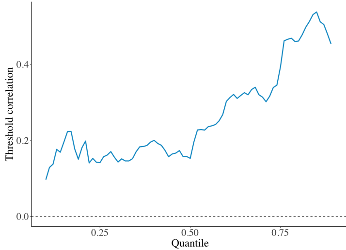
Figure 5.2: Threshold correlation of GARCH(1,1) standardized returns (training period).
