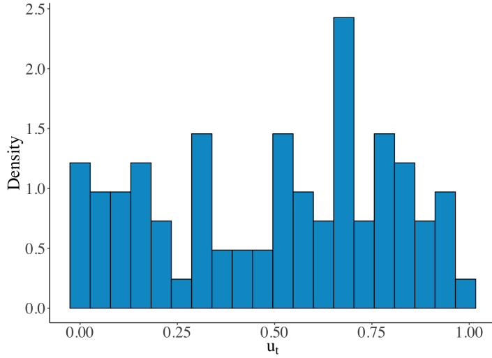
Figure 4.8: Histogram of PIT values, GJR- Asyt.
