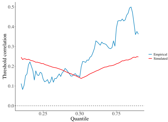
Figure 5.4: Empirical and simulated threshold correlations of GJR-GJR copula.
