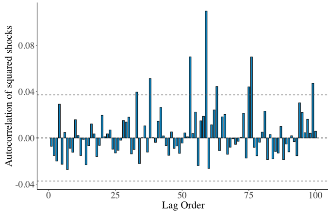
Figure 4.2: Autocorrelation of squared returns over variance (2014-2024), GJR-GARCH(1,1).
