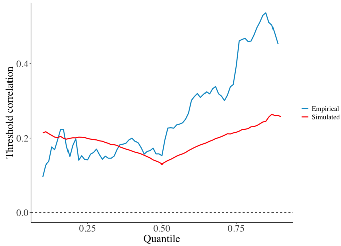
Figure 5.3: Empirical and simulated threshold correlations of GARCH-GARCH copula.
