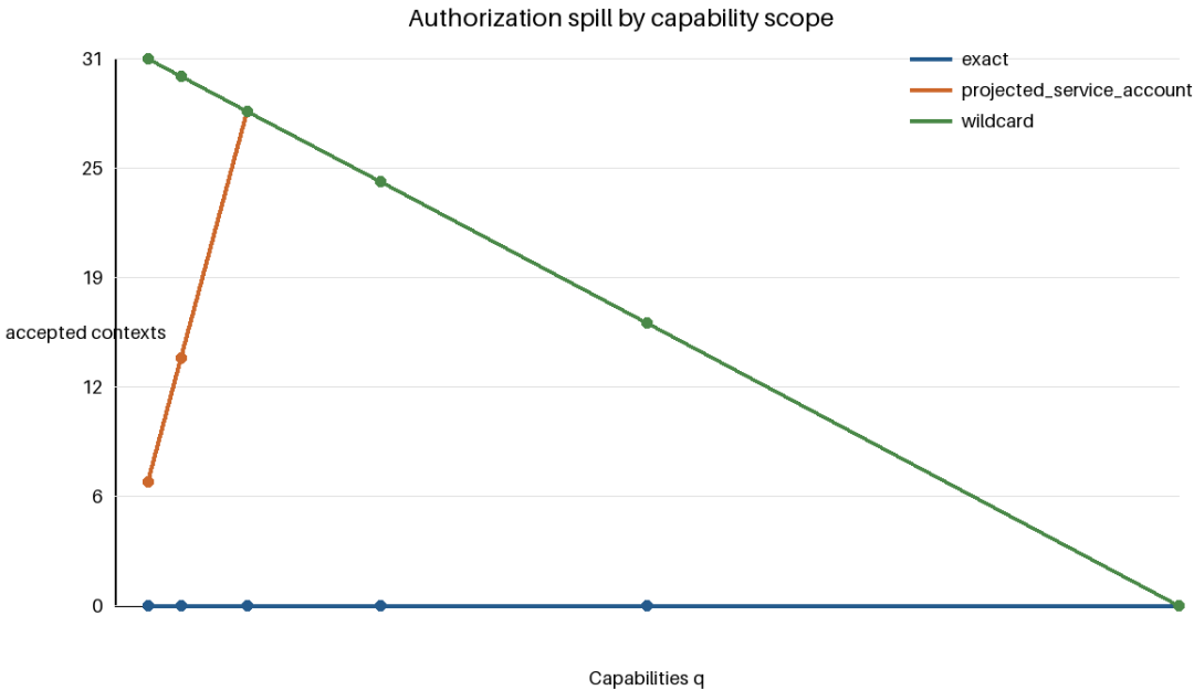
Figure 2. Authorization spill in the 32-context experiment. Exact binding remains at zero; broader bindings admit the contexts their omitted fields leave unconstrained.
