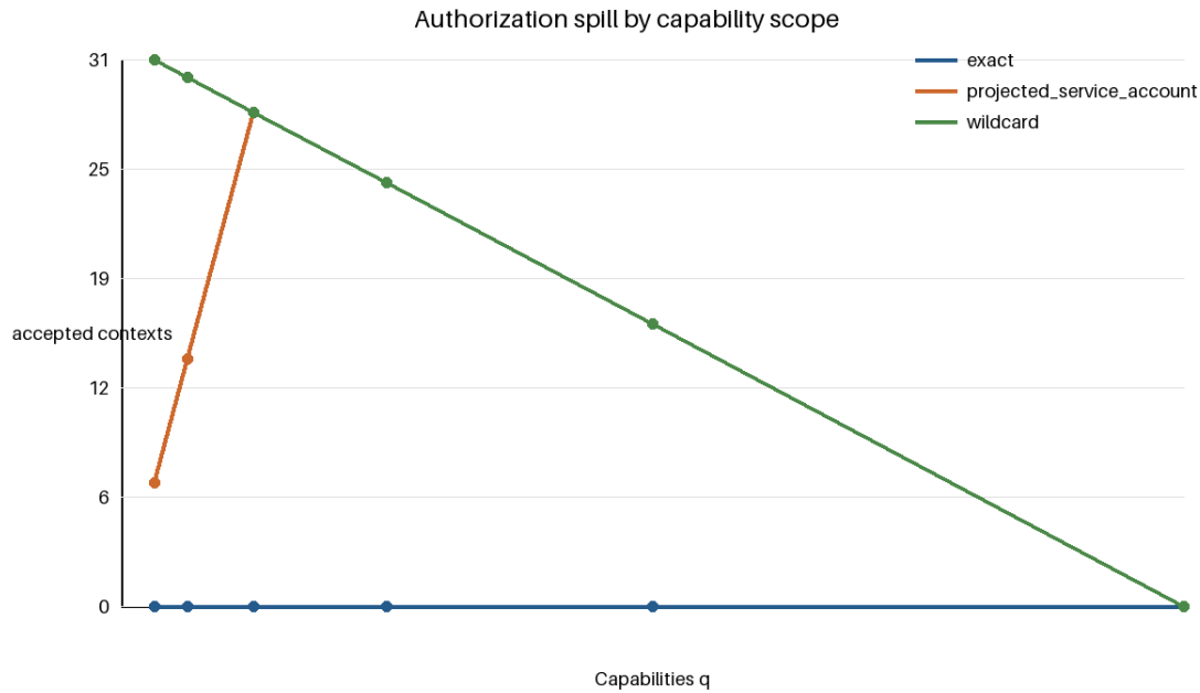
Authorization spill under exact, projected, and wildcard capability scopes.
