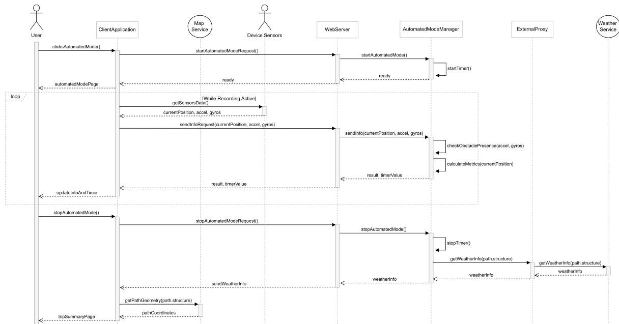
Figure 16: [SD10] Automated Mode Sequence Diagram
