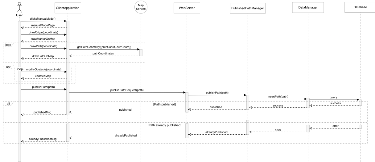
Figure 15: [SD9] Publish Path Sequence Diagram
