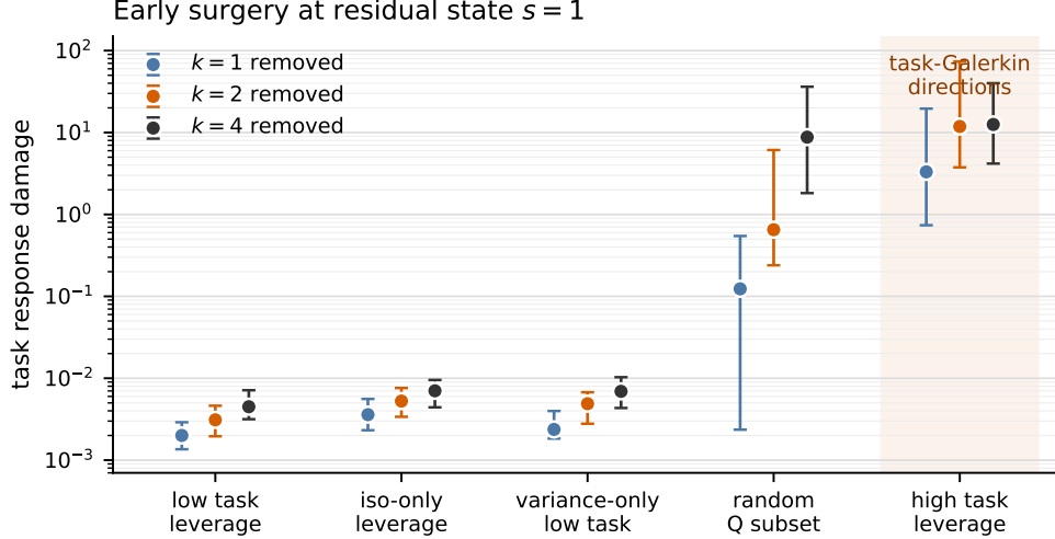
Figure 4: Experiment 3: causal effect of task-important activation directions. Task finite-difference response damage after removing k context-token directions at residual state s = 1 . High task-leverage directions produce orders-of-magnitude larger damage than low-task-leverage directions from the same activation basis.
