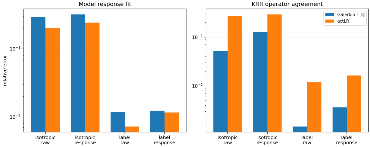
Figure 1: Experiment 1 reduced-operator certificate versus same-span response fitting. The response-fitted operator can fit the transformer slightly better on task probes, but the KRR-constrained reduced operator is much closer to exact KRR.
