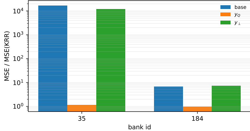
Figure 7: Experiment 4 target-rich outliers. Feeding y_Q = AQQ^{\top}y repairs the two bad episodes; feeding y_{\perp} = y - y_Q does not.
