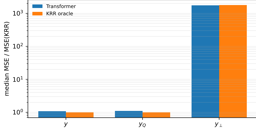
Figure 6: Experiment 3 on-manifold label-space projection. The transformer and KRR oracle both remain near the original KRR error on y_Q , while both fail on y_{\perp} .
