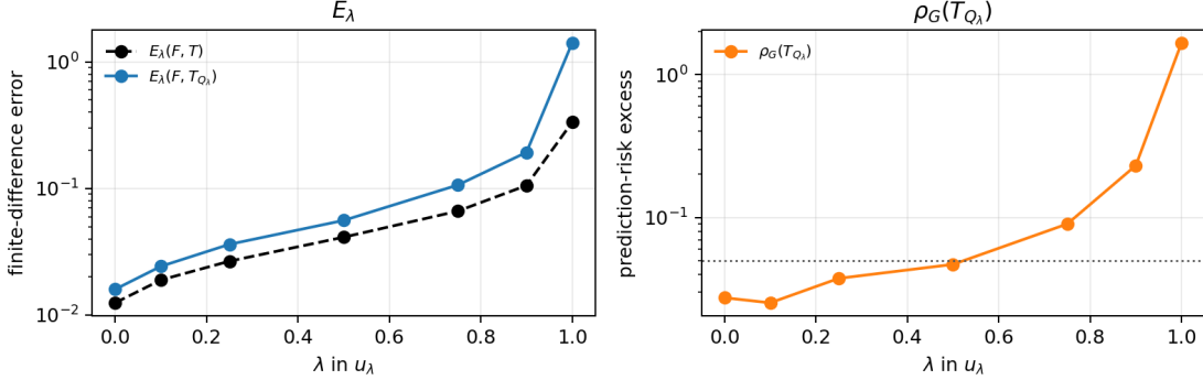
Figure 3: Experiment 1 task-to-isotropic probe interpolation with matched response bases. For each \lambda , Q_\lambda is built from the same mixed perturbations used in the plotted errors. Left: finite-difference response errors on the mixed probe law. Right: task prediction-risk excess \rho_G(T_{Q_\lambda}) , with the dotted line marking the five-percent tolerance. As \lambda approaches 1, even the matched response basis no longer supports a clean KRR-constrained explanation.
