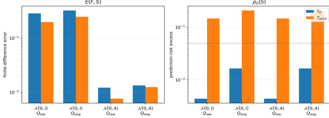
Figure 2: Experiment 1 same-span readout control. Left: finite-difference response error E(F, S) on task and isotropic probes. Right: prediction-risk excess \rho_G(S) , with the dotted line marking the five-percent tolerance. T_Q and actLR use the same activation coordinates Q^\top u . actLR fits the transformer’s finite-difference responses with a free least-squares readout; T_Q uses the KRR-constrained readout K_t Q .
