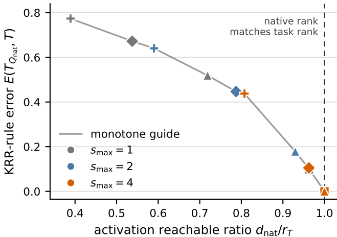
A. Activation rank threshold for KRR rule
